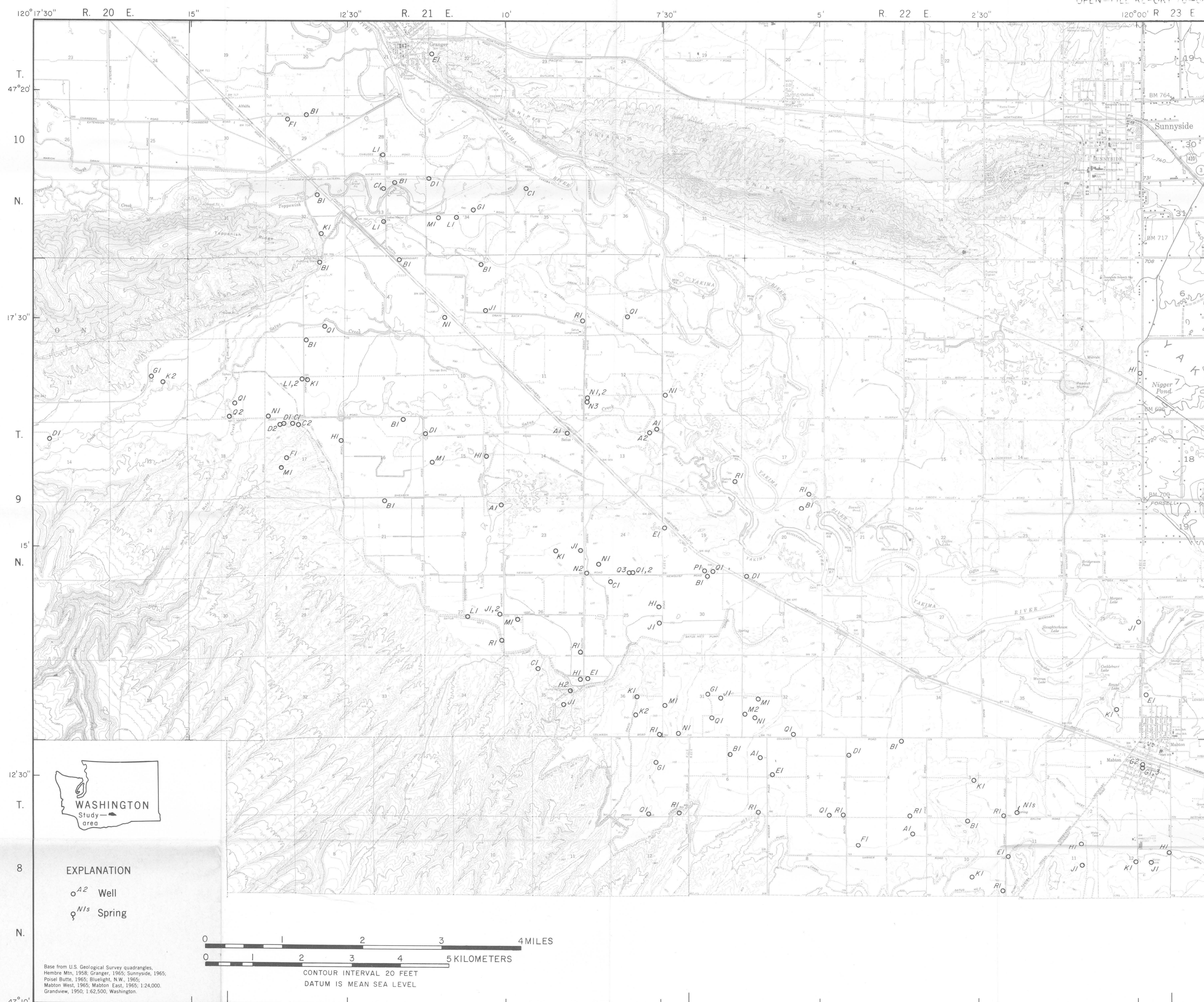
PLATE 1 -- Locations of wells in lowland of Satus Creek basin.
