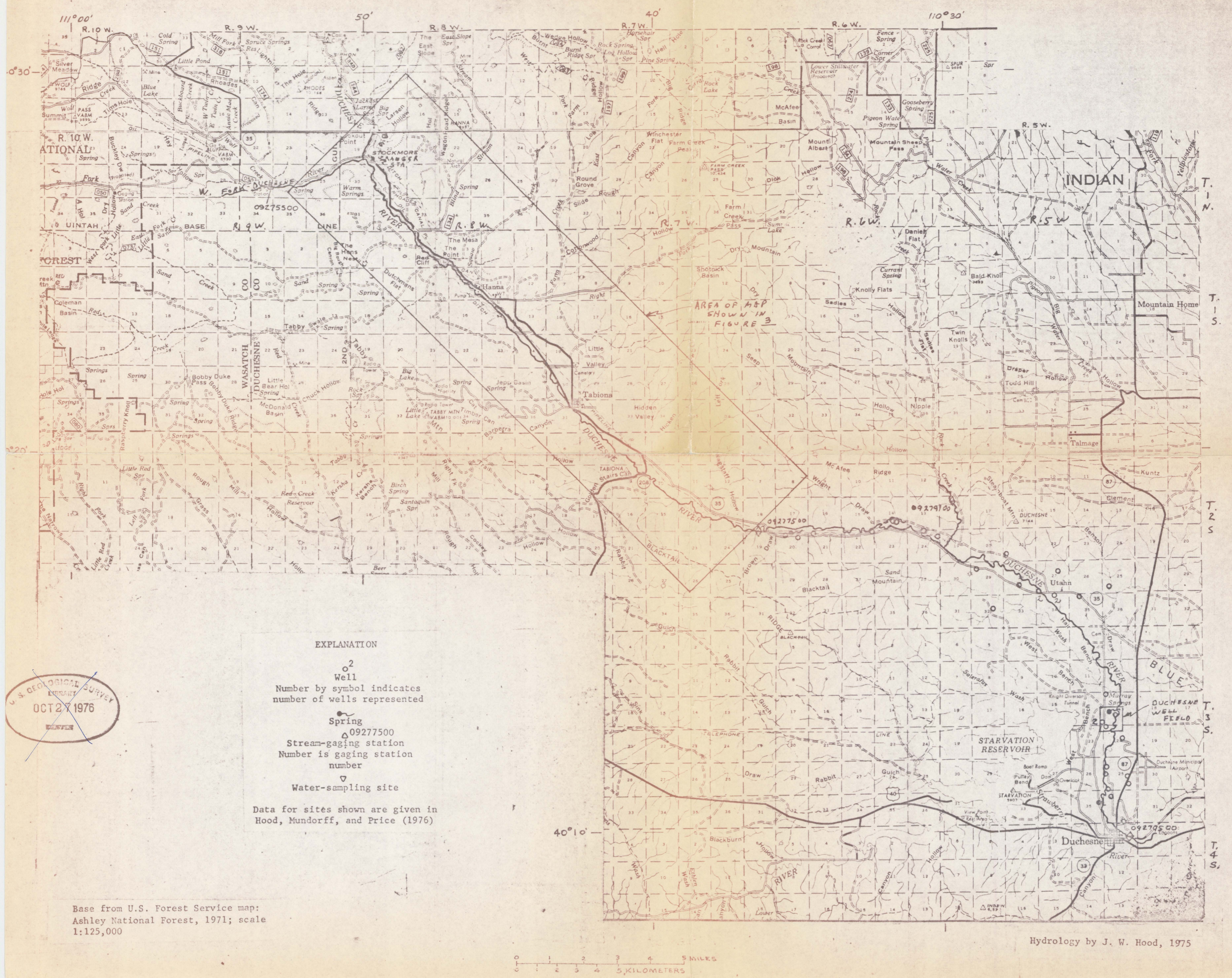
Figure 2.--Selected hydrologic data in the upper Duchesne River valley and adjacent area.
