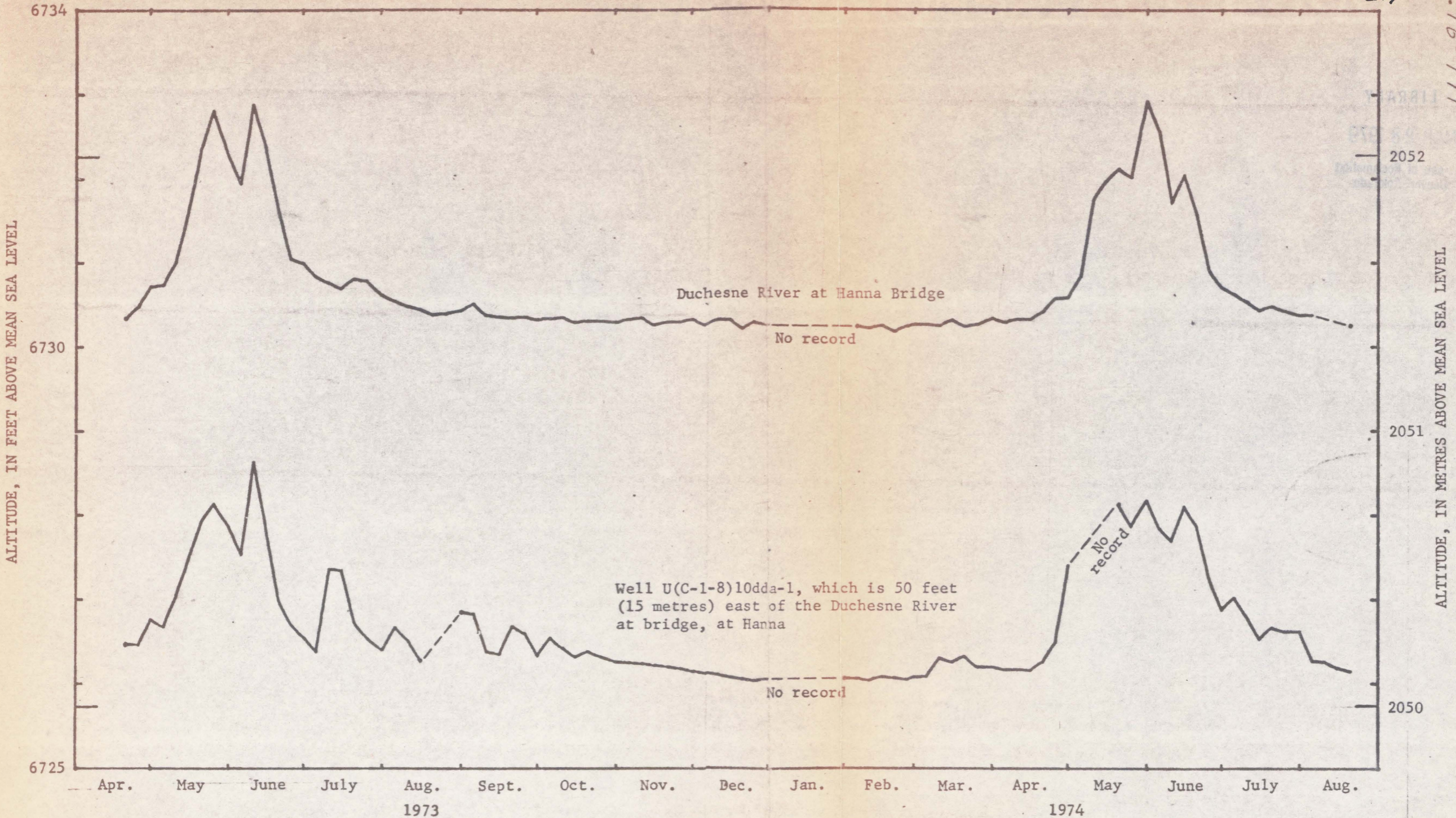
Figure 5.--Stage of the Duchesne River at Hanna Bridge (data-site (154) and water level in well U(C-1-8)10dda-1, 1973-74.
