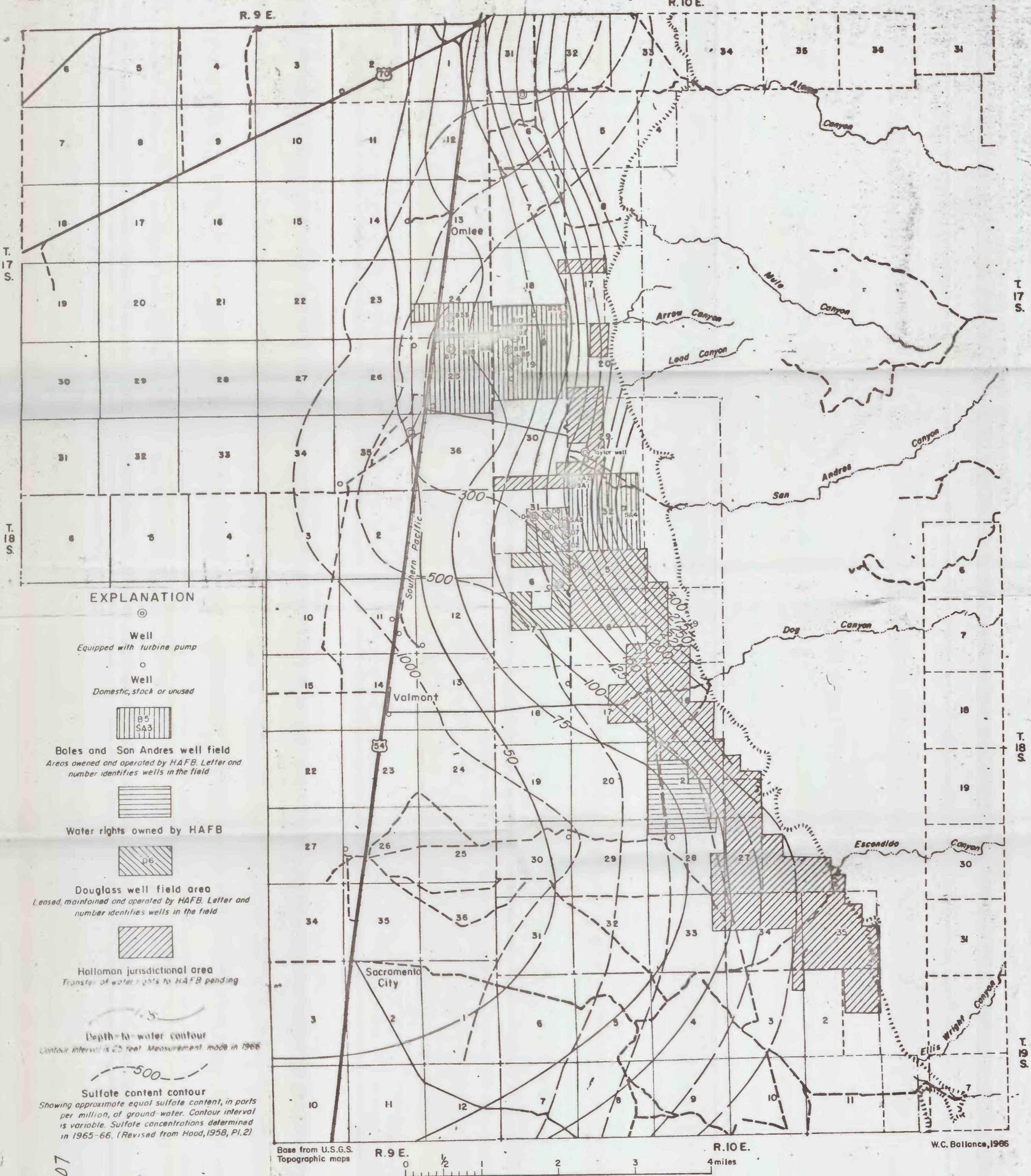
Figure 6.--Approximate sulfate content of ground water and depth-to-water map (showing location of wells and well-field areas), Holloman Air Force Base, Otero County, New Mexico.
