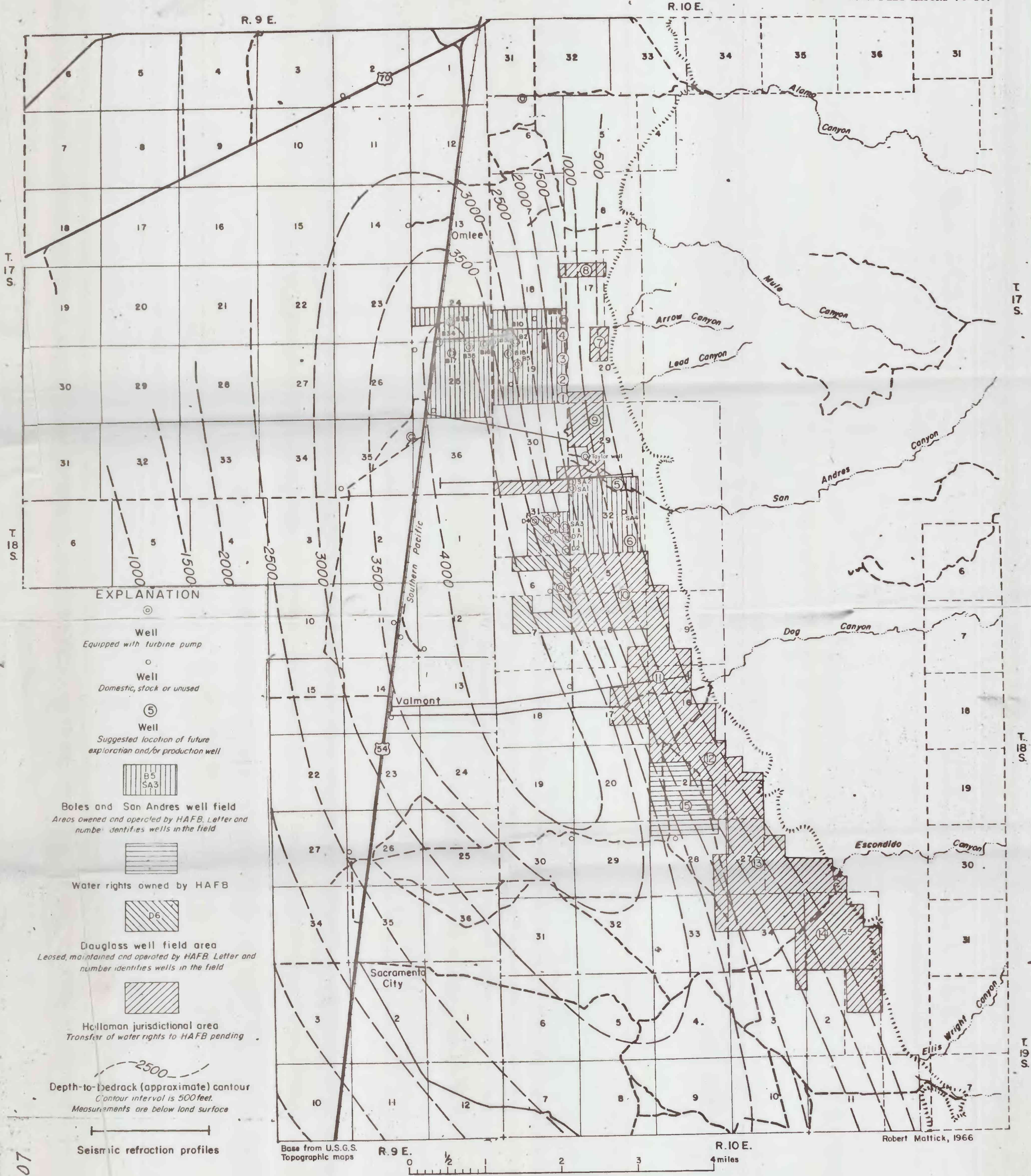
Figure 15.--Approximate depth to bedrock (thickness of unconsolidated material), location of wells, and well-field areas, Holloman Air Force Base, Otero County, New Mexico.
