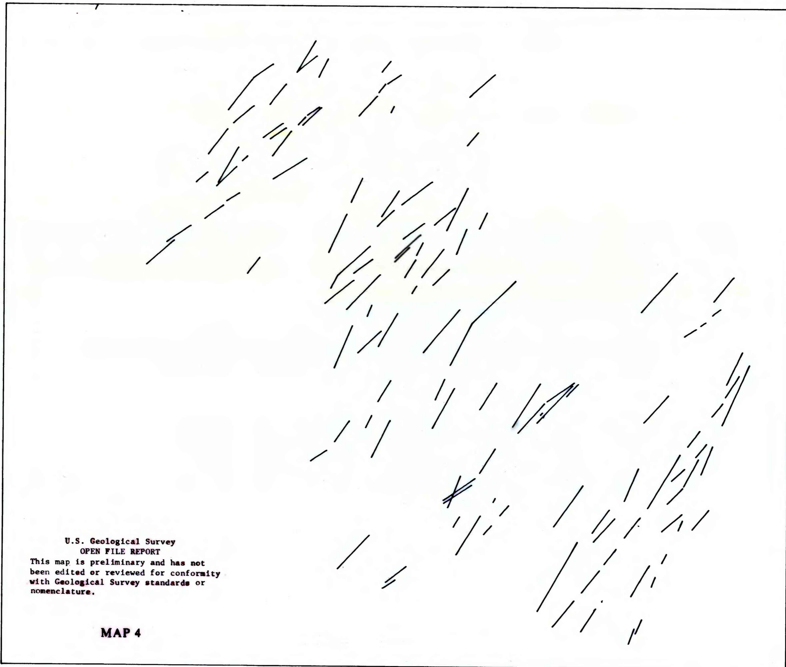
SONORA LINEAMENTS, SIOUX FALLS IMAGE 1:1,000,000 BAND 5 20-57 TREND
