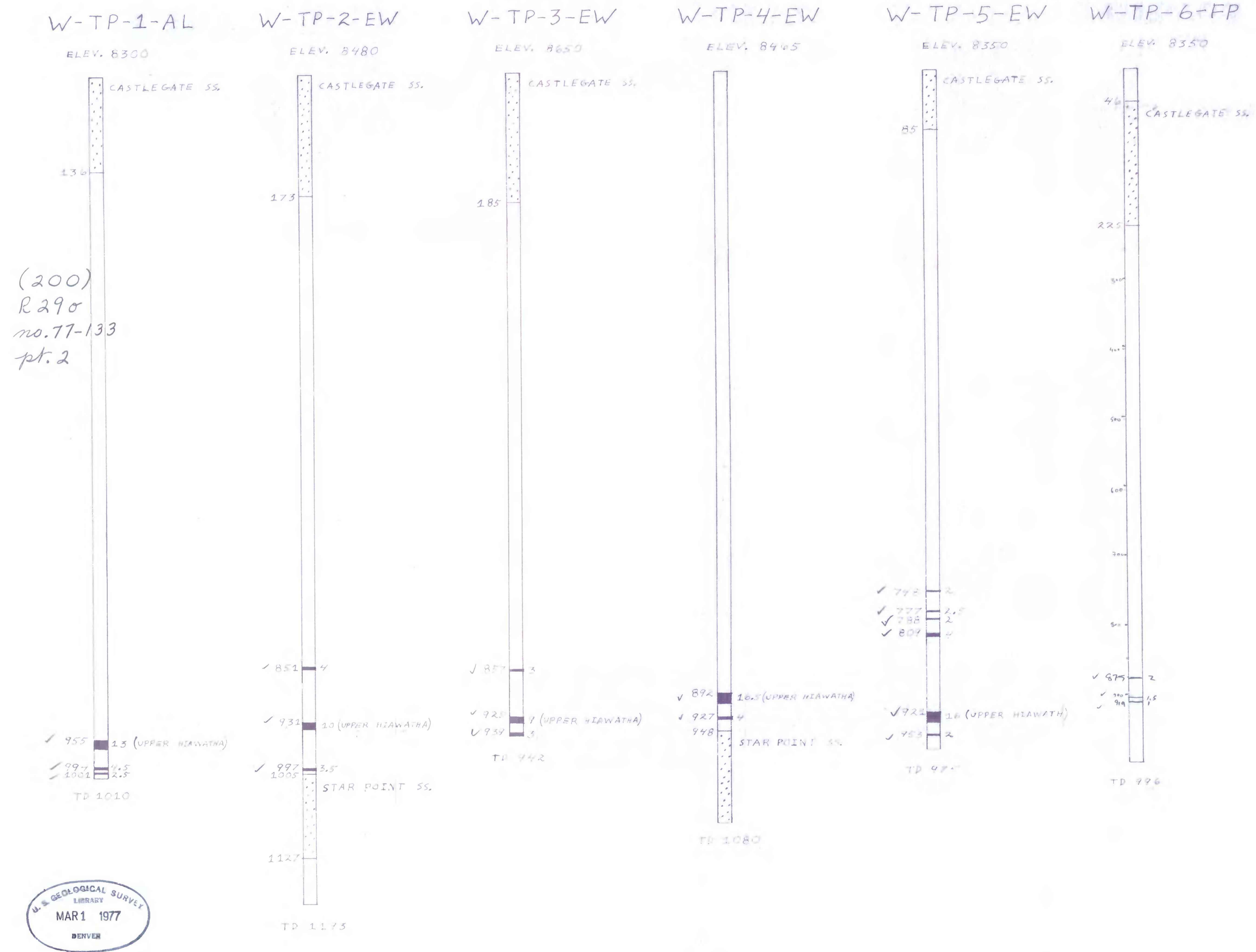
FIGURE 7 COAL SECTIONS FROM HOLES DRILLED IN THE PINES AREA, UTAH
