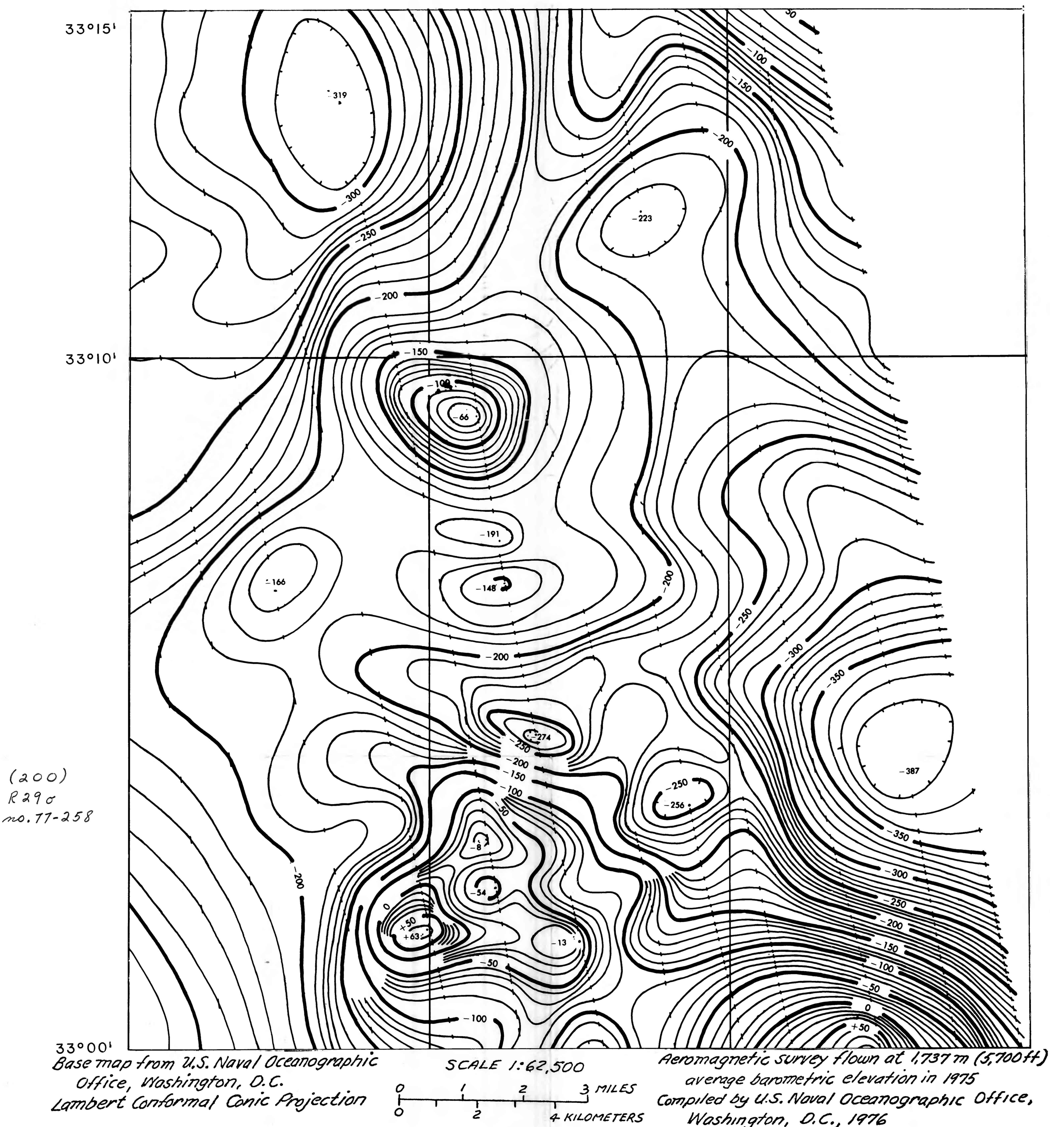
FIGURE 4.--AEROMAGNETIC MAP OF TULAROSA 15-MINUTE QUADRANGLE, NEW MEXICO 1977
