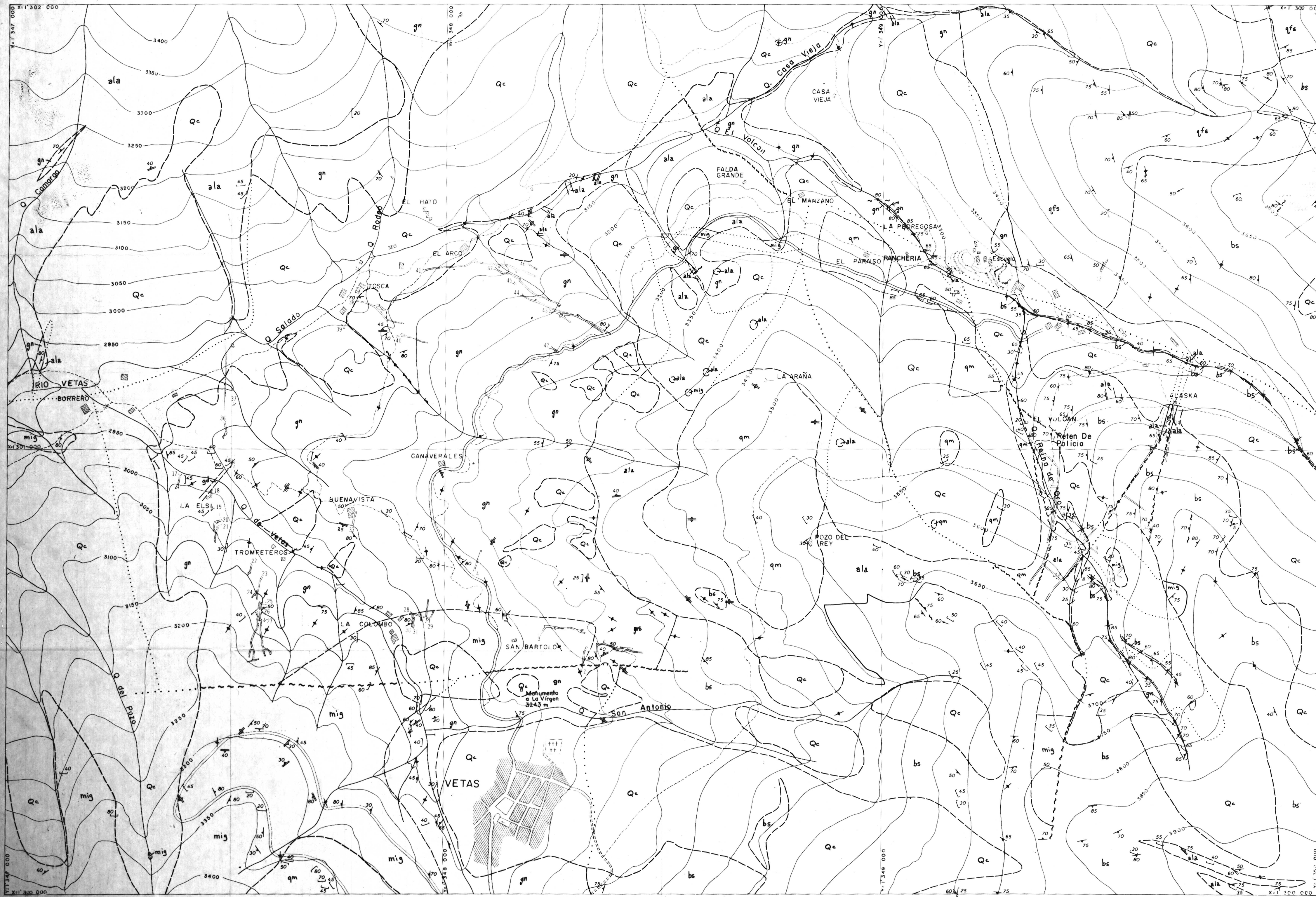
FIGURE 4. PRELIMINARY GEOLOGIC MAP OF THE VETAS DISTRICT, COLOMBIA
