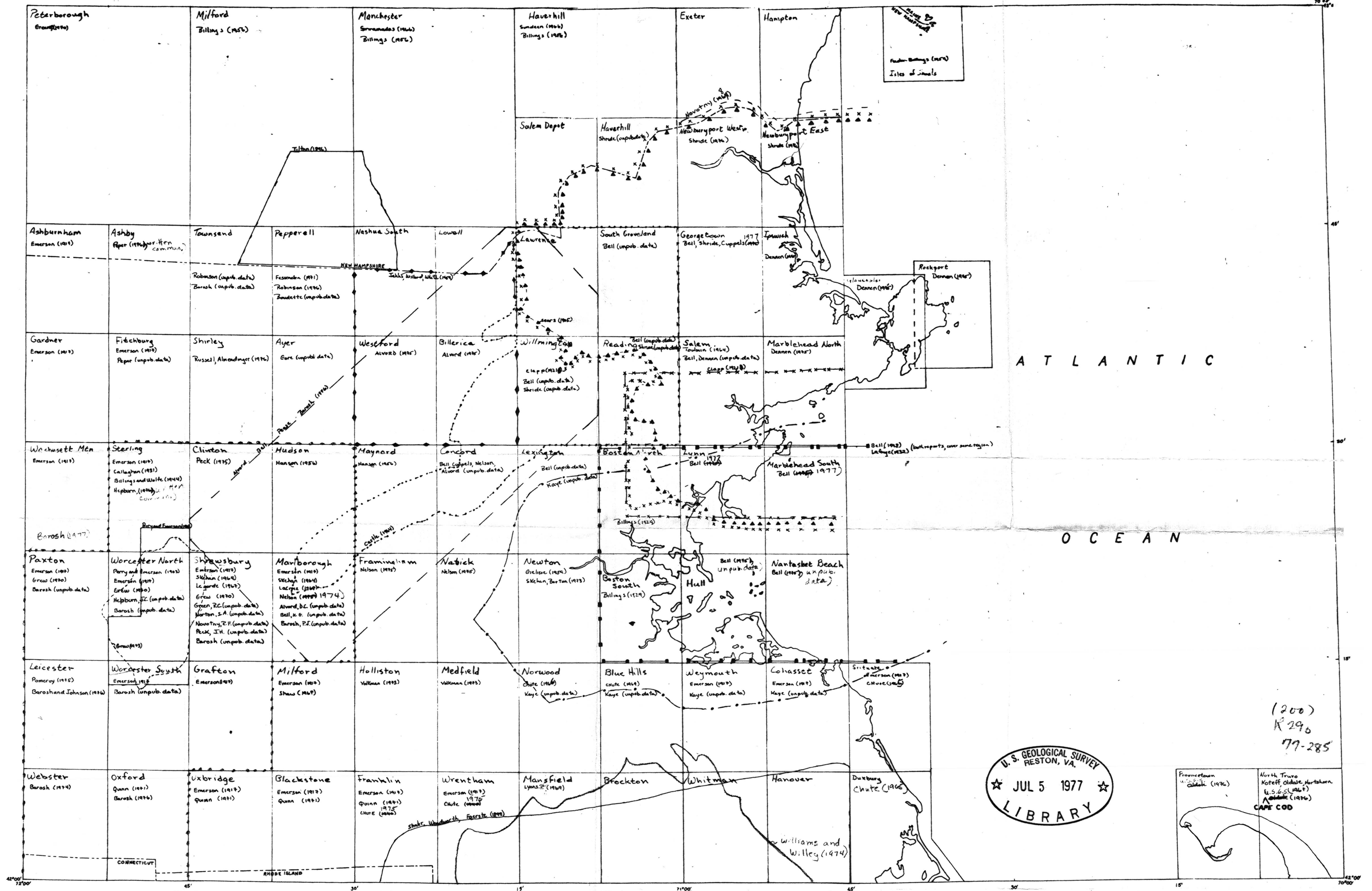
INDEX TO GEOLOGIC MAPS USED IN THE COMPILATION OF THE BOSTON 2° SHEET
