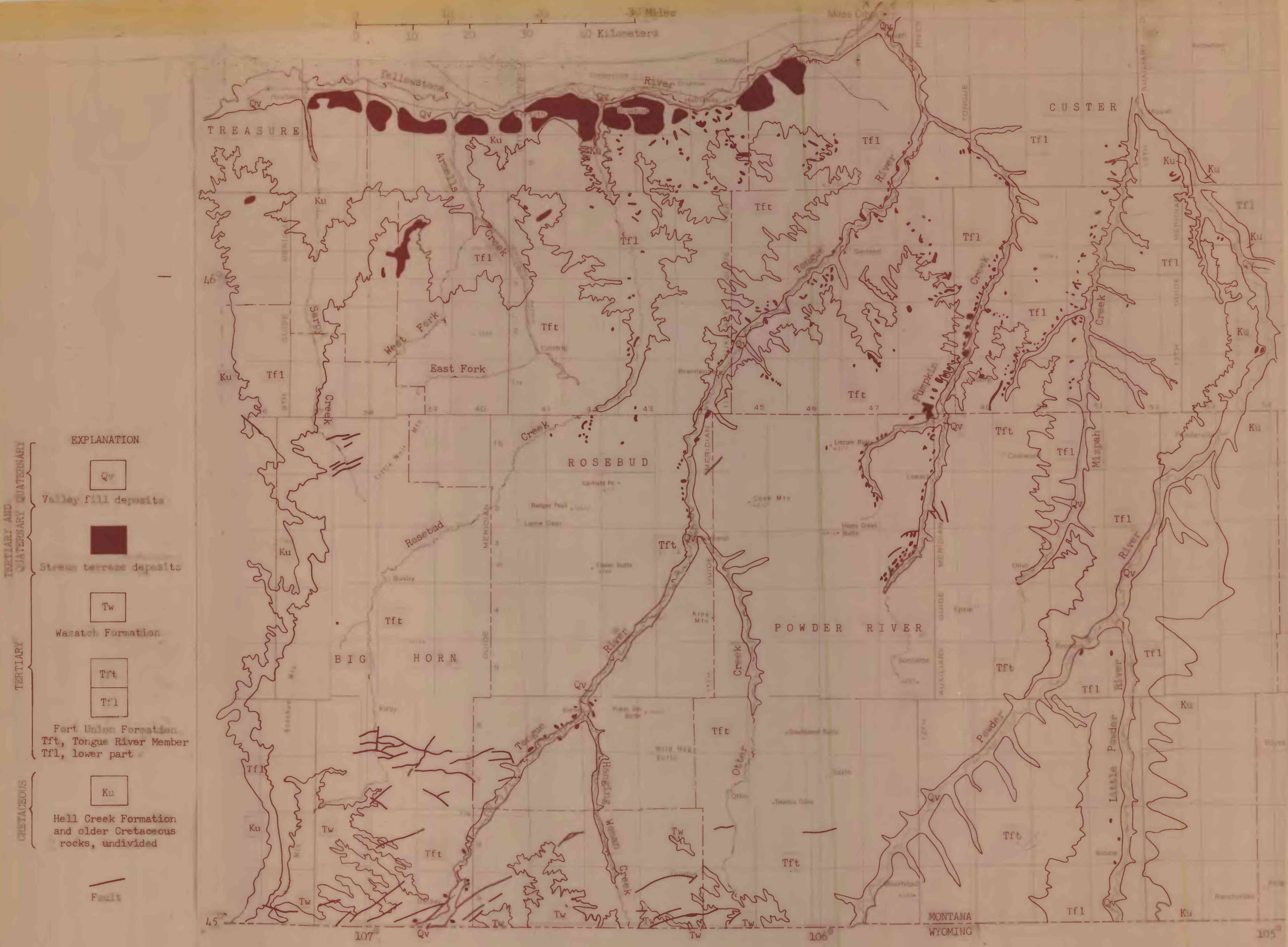
Figure 6. Geologic map of the northern Powder River coal region, Montana
