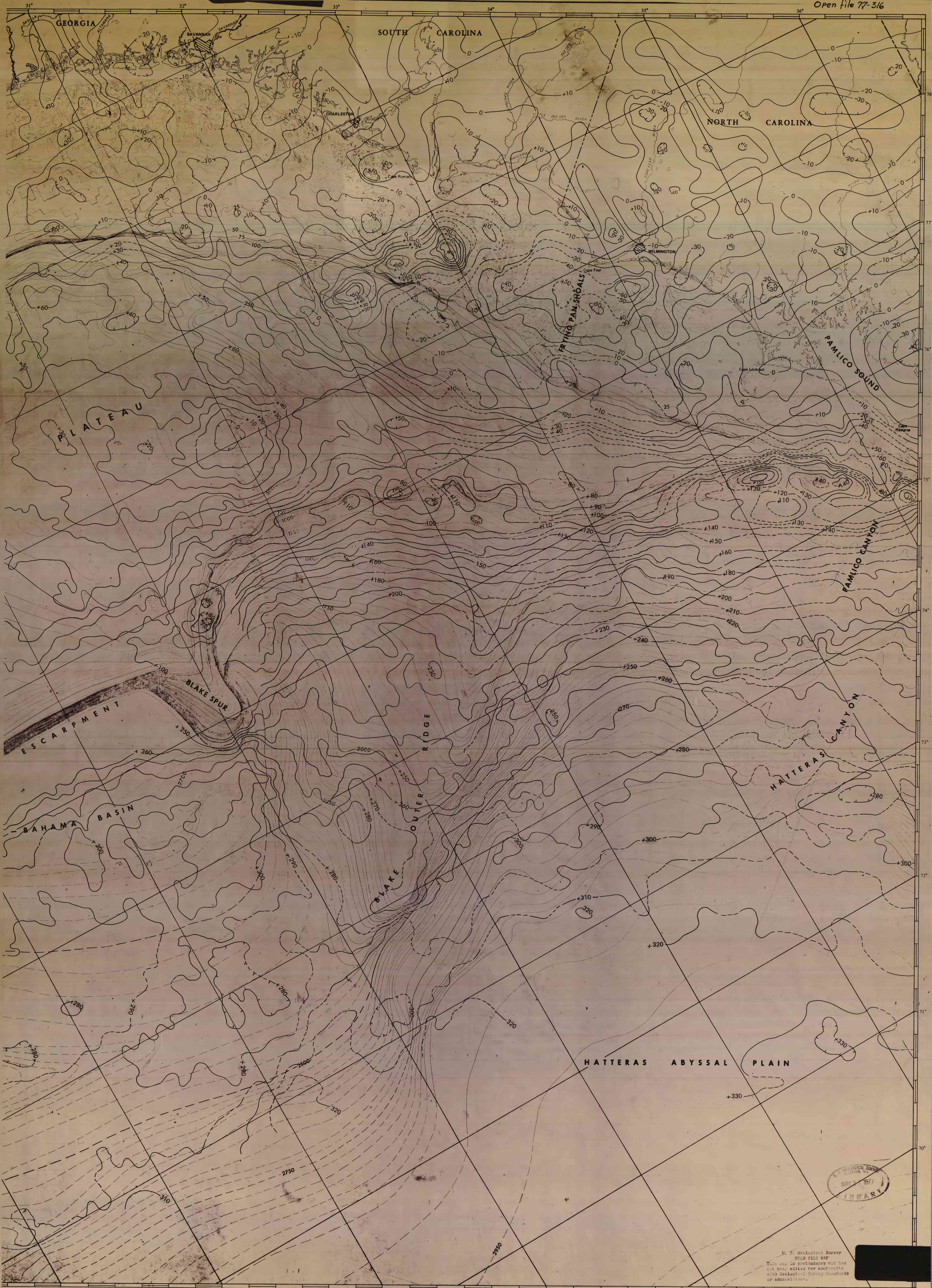
SIMPLE BOUGUER ANOMALY REPRESENTATION OVER A PART OF THE ATLANTIC CONTINENTAL SHELF AND ADJACENT LAND AREAS OF GEORGIA, THE CAROLINAS AND NORTHERN FLORIDA
