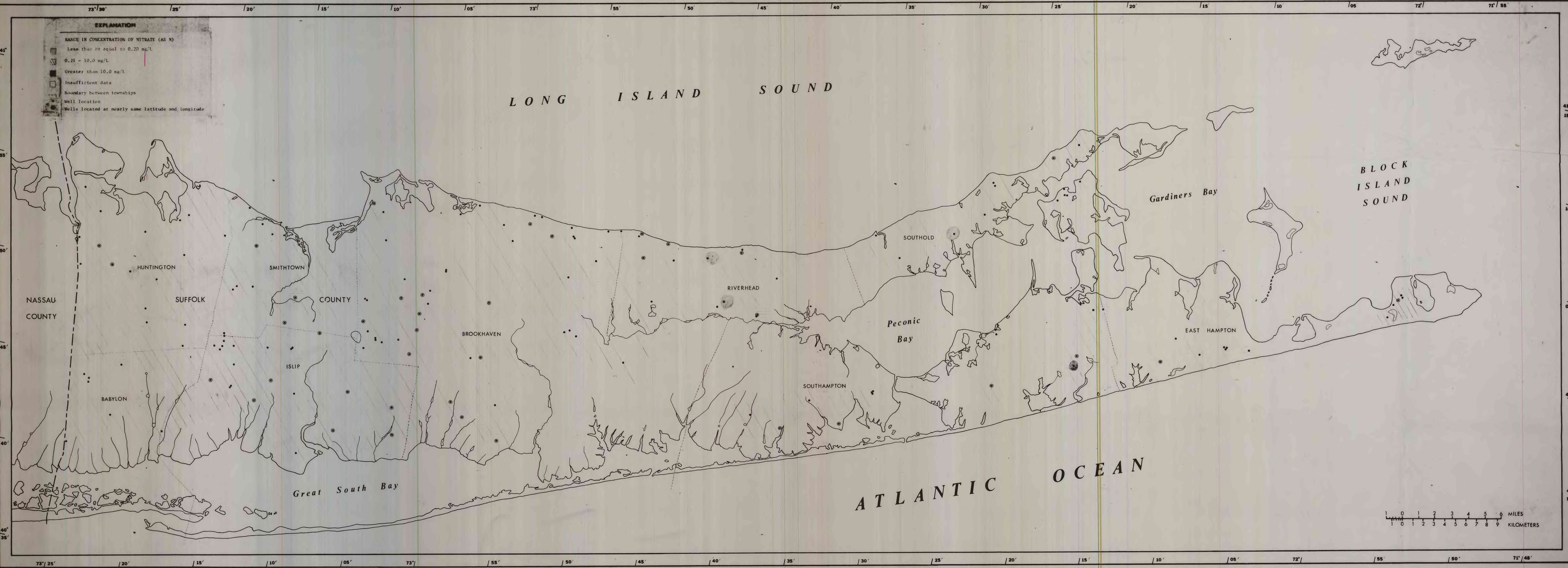
Figure 2.—Areal distribution of nitrate concentrations (as N) in the upper glacial aquifer, Suffolk County
