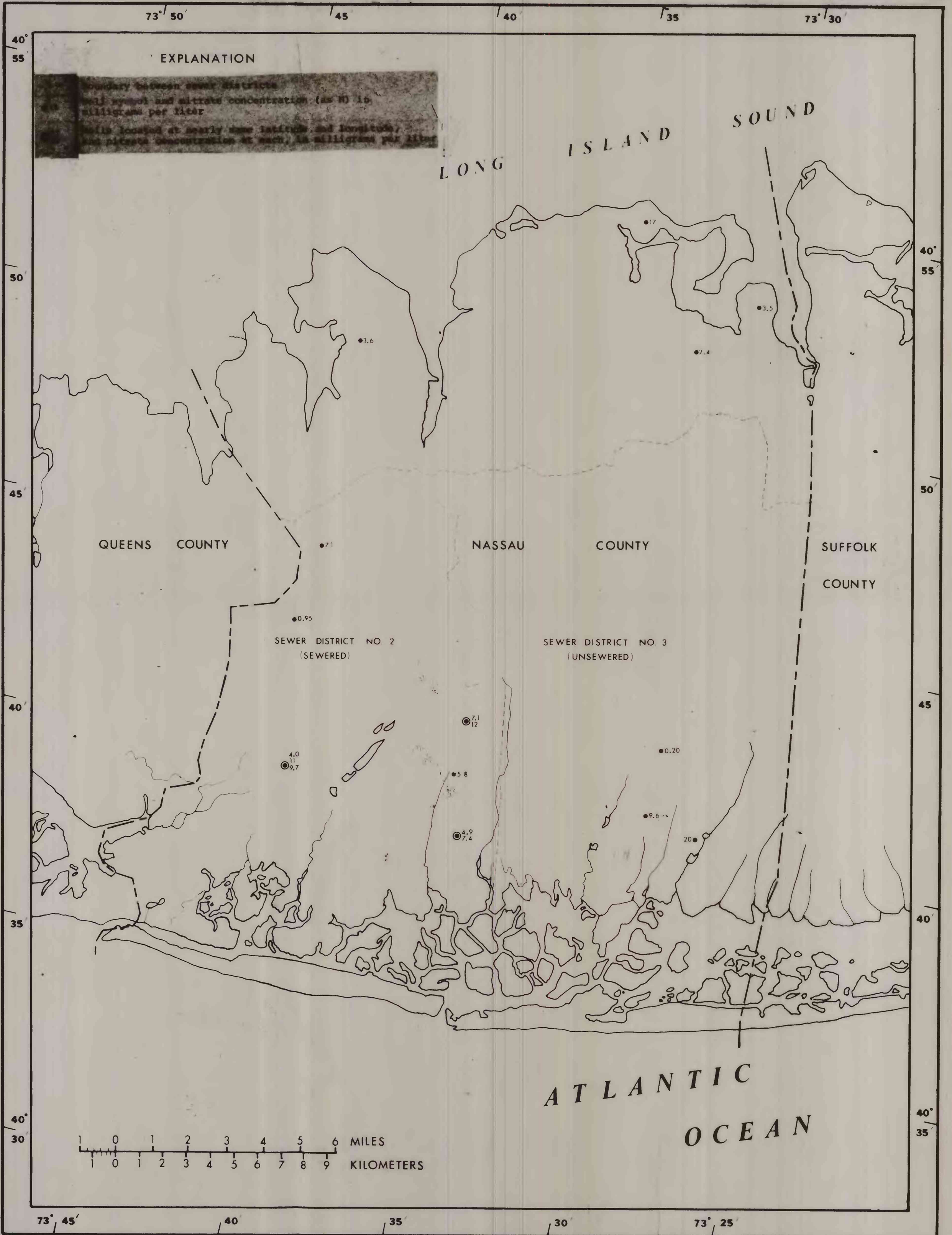
Figure 3.--Areal distribution of nitrate concentrations (as N) in the upper glacial aquifer, Nassau County
