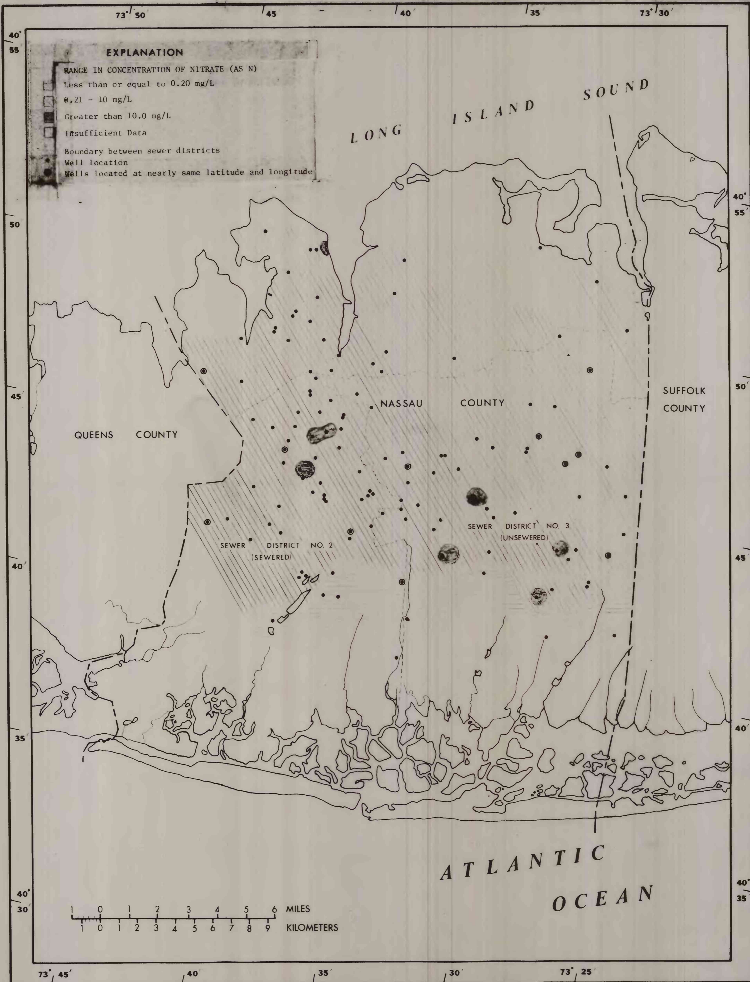
Figure 4.--Areal distribution of nitrate concentrations (as N) in the Magothy aquifer, Nassau County
