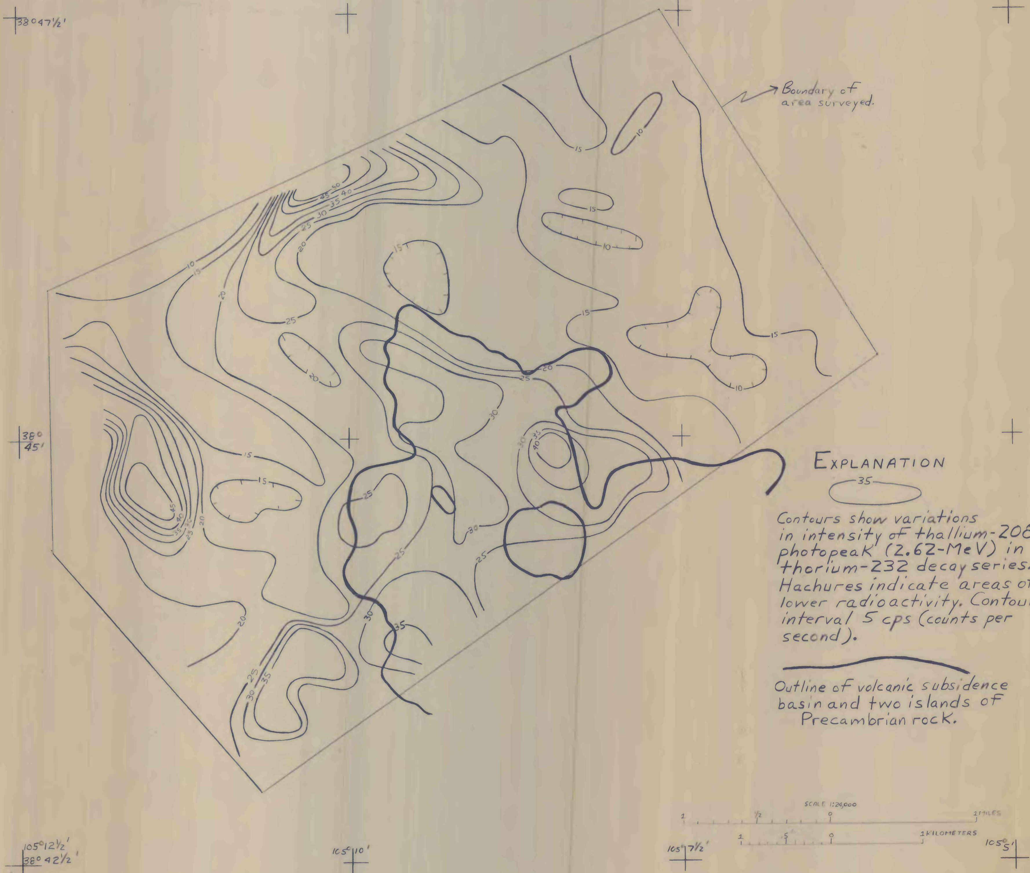
Plate IV. Contour map of equivalent thorium distribution in part of the Cripple Creek district, Colorado.
