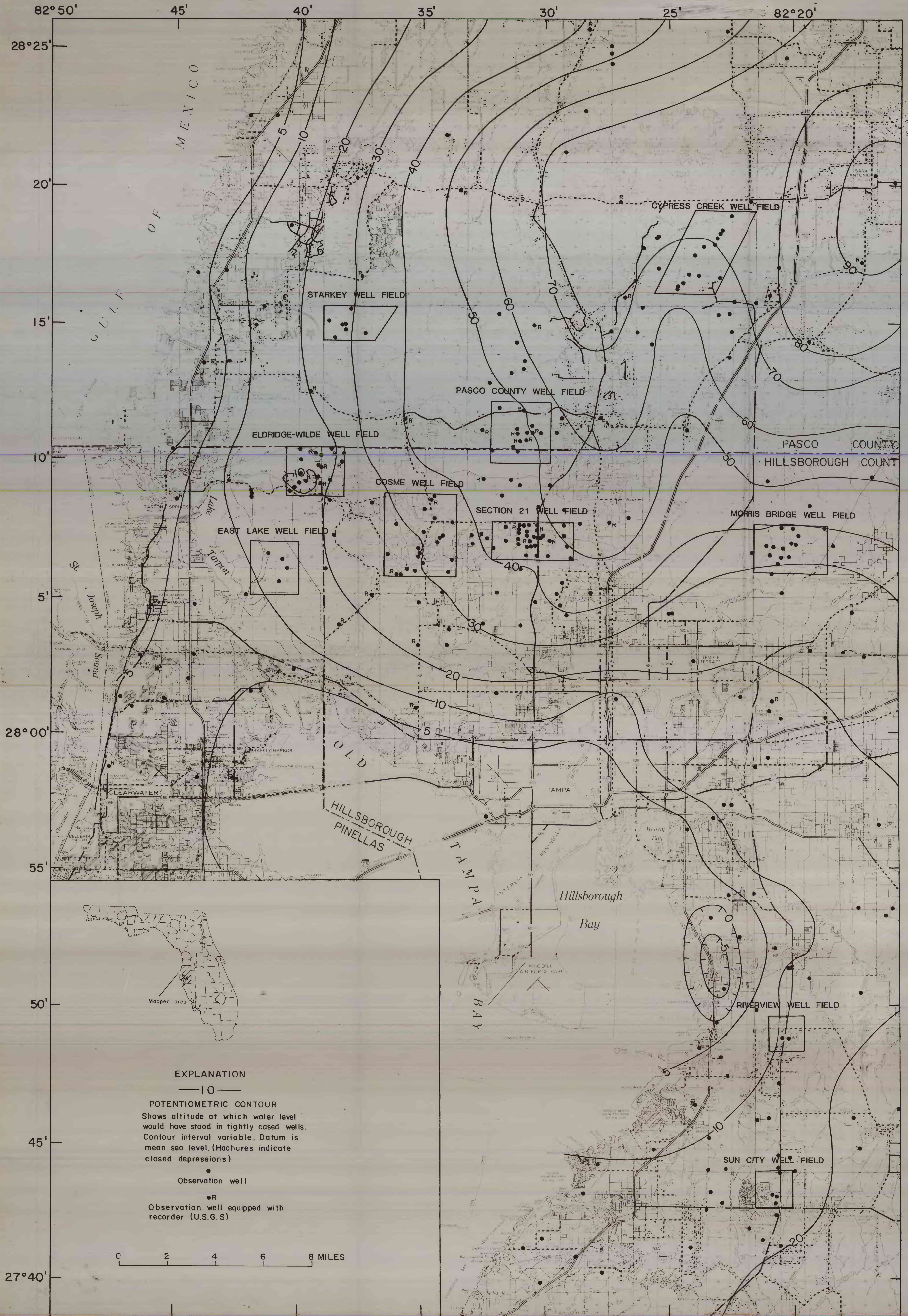
POTENTIOMETRIC SURFACE OF FLORIDAN AQUIFER, WEST-CENTRAL FLORIDA, SEPTEMBER 1976, BY P.D. RYDER AND L.R. MILLS
