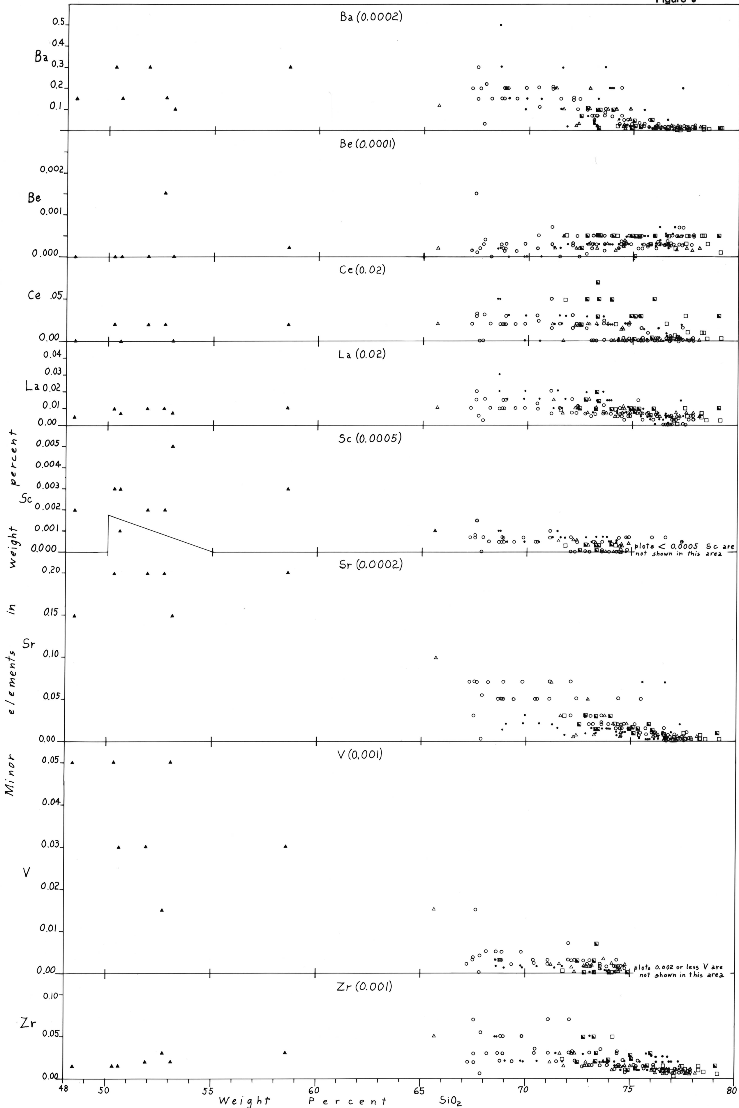
Figure 5.--Synoptic silica variation diagrams for selected minor elements in igneous rocks from the Timber Mountain-Oasis Valley caldera complex. Symbols for these rocks are the same as those on figure 4. Threshold limits of detection are indicated for individual elements in parentheses; less-than-threshold determinations are plotted arbitrarily as zero except for some values that were determined under favorable conditions. SiO_2 values from analysis recalculated volatile free.
