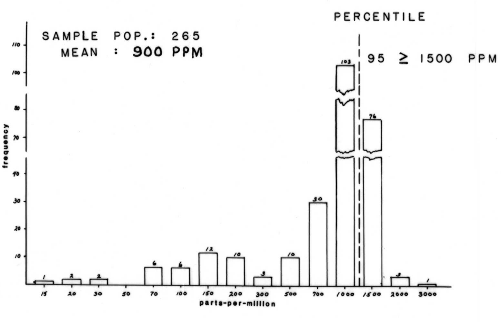
HISTOGRAM HISTOGRAM OF GEOCHEMICAL ABUNDANCE DERIVED FROM RESULTS OF SEMIQUANTITATIVE EMISSION SPECTROGRAPHIC ANALYSES OF SELECTED ROCK SAMPLES FROM THE RED MOUNTAIN ULTRAMAFIC BODY (RM) REPORTED BY CLARK, GRYBECK, GREENWOOD, AND OTHERS (1978).
