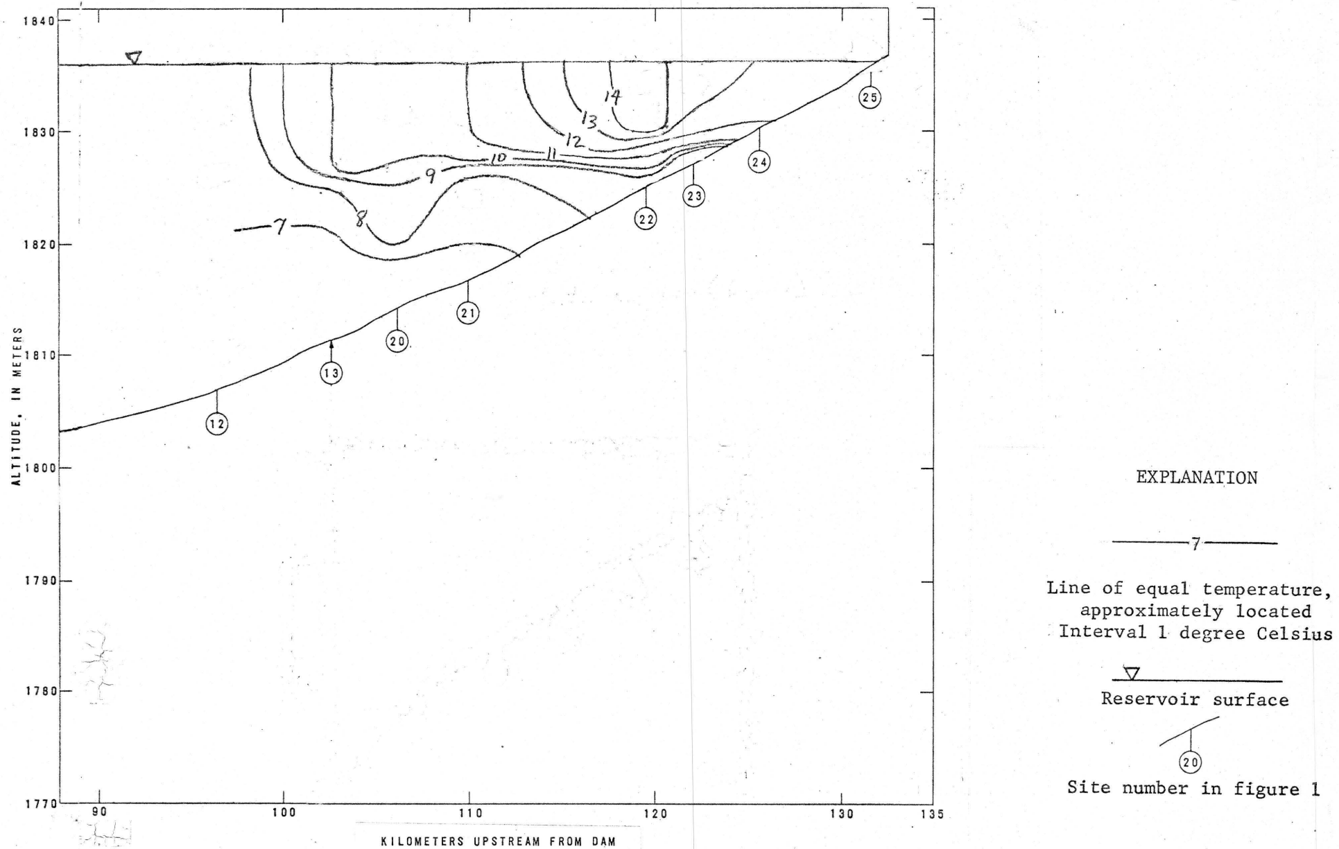
Figure 3.--Longitudinal temperature profile of the upstream part of Flaming Gorge Reservoir, May 1975.
