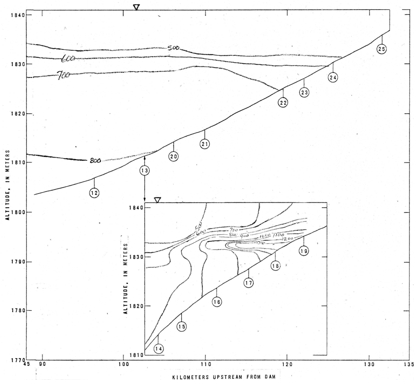
Figure 8.--Longitudinal profile of specific conductance in the upstream part of Flaming Gorge Reservoir, July 1974.
