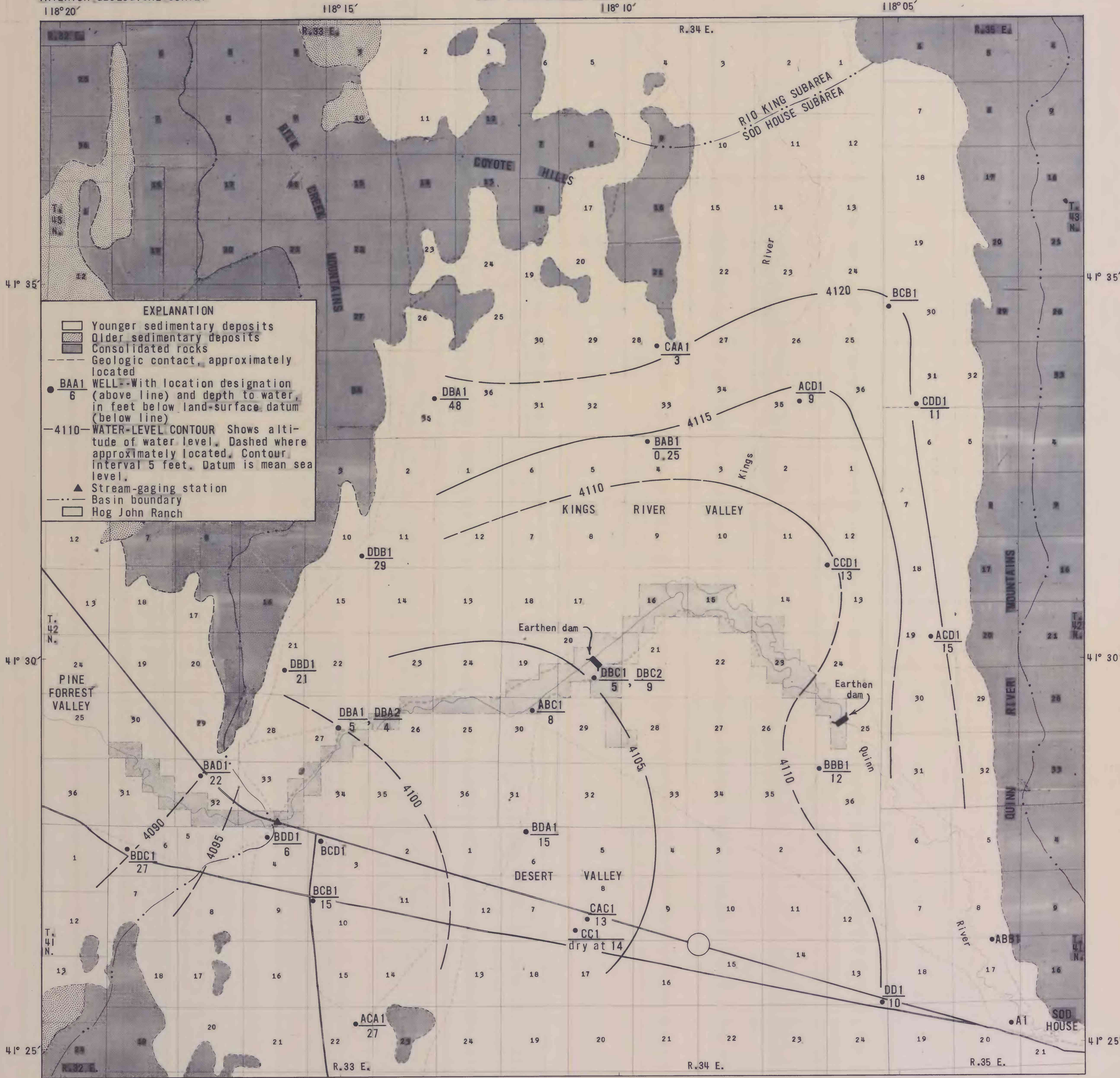
1 1/2 0 1 2 3 Miles PLATE 3.--GENERAL GEOLOGY, WELL LOCATIONS, DEPTH TO WATER, AND WATER-LEVEL CONTOURS IN THE VICINITY OF HOG JOHN RANCH, MARCH 1976.
