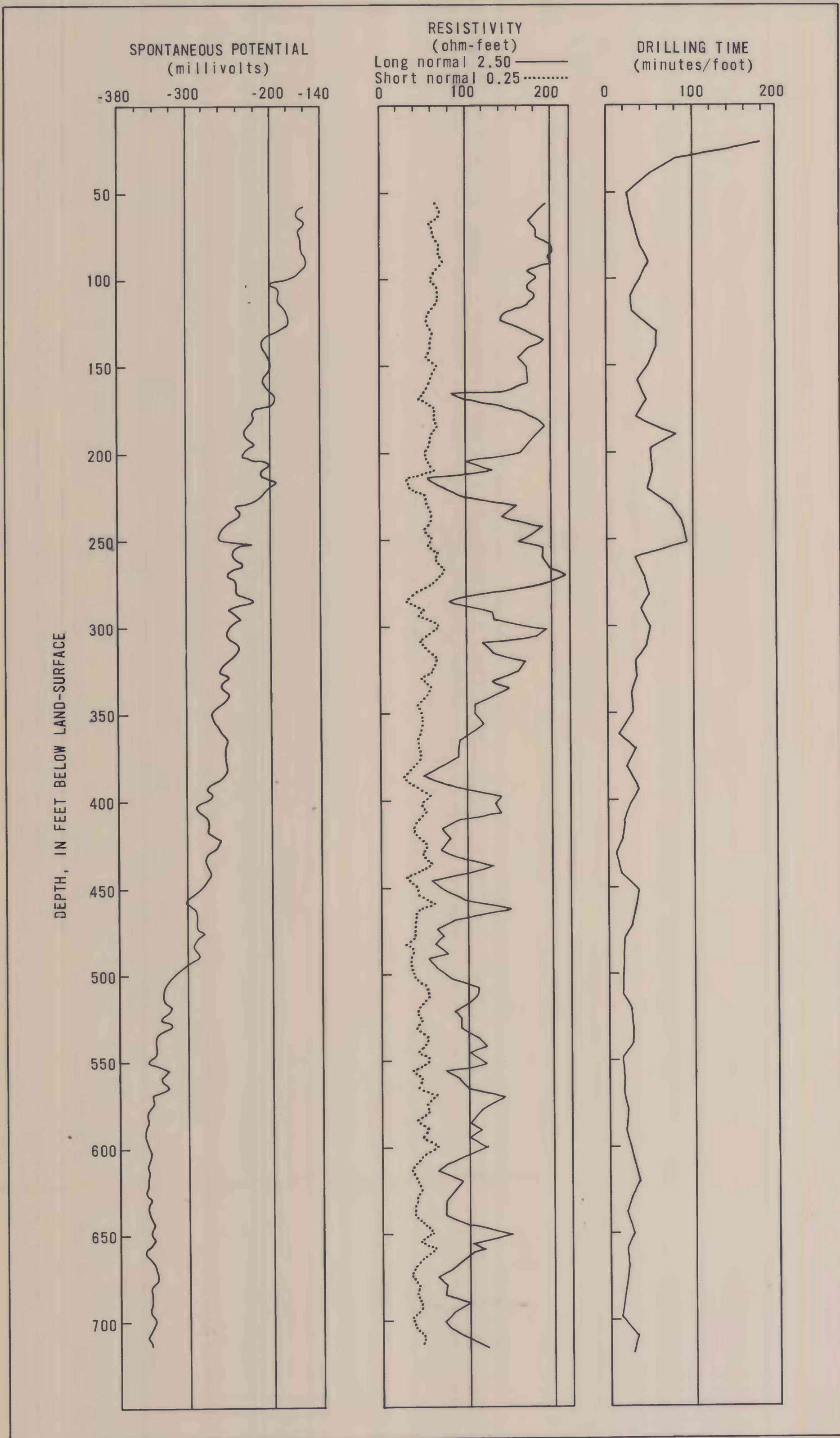
PLATE 4.--ELECTRIC LOGS AND DRILLING-TIME LOG FOR TEST WELL 33B N47 E38 21DAA1.
