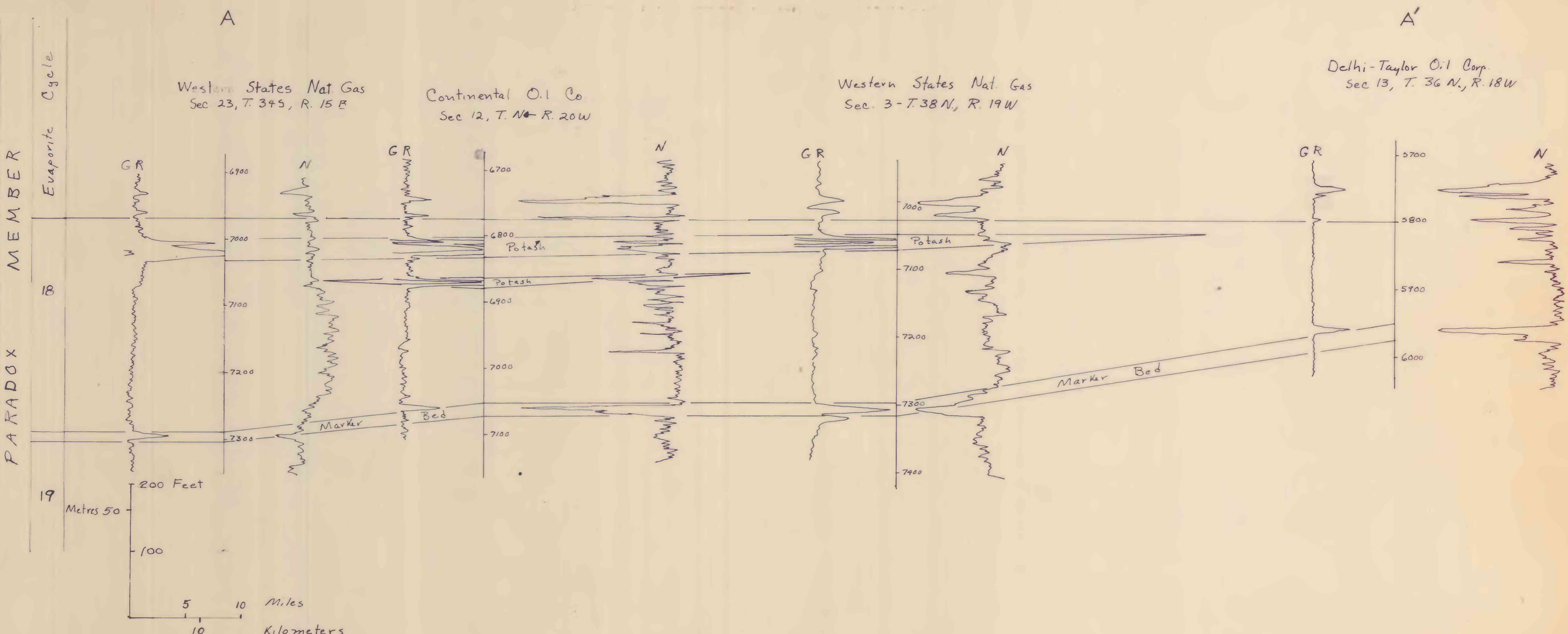
Figure 2 - Geophysical log correlation of evaporite cycle 18 of section A-A' shown on figure 1.
