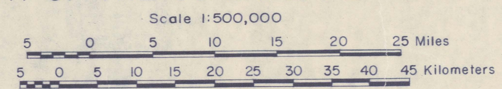
MAP 2 AEROMAGNETIC MAP OF PART OF THE COASTAL PLAIN REGION OF NORTH CAROLINA
