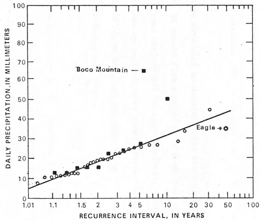
Figure 11.--Frequency curve of maximum daily precipitation at Eagle for the summer months and maximum daily precipitation recorded at Boco Mountain.
