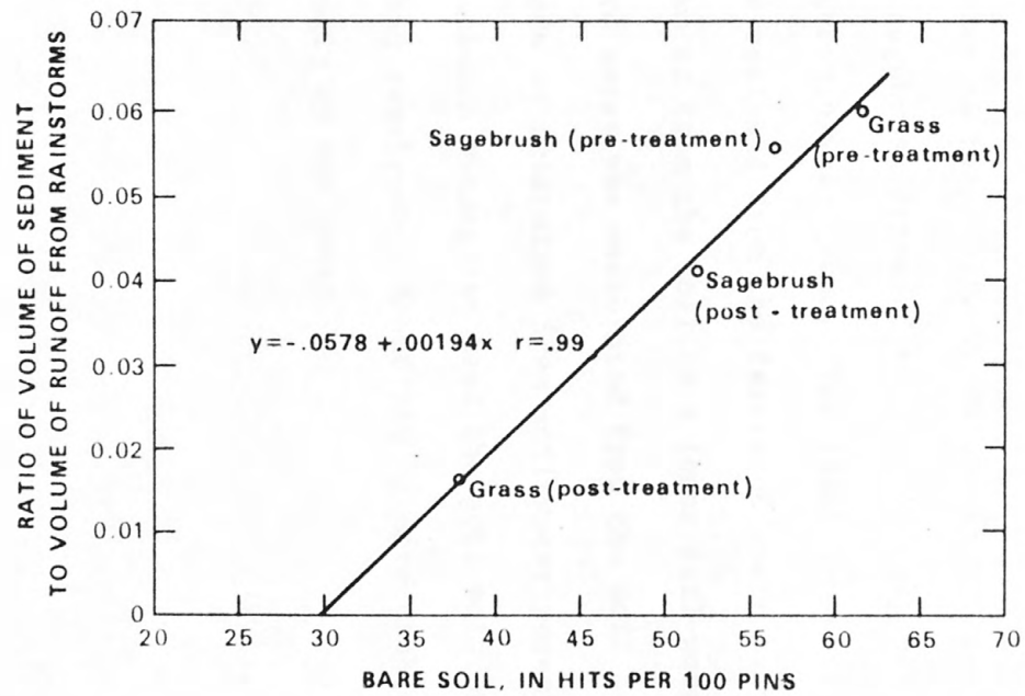
Figure 16.--Relationship between the ratio sediment yield/runoff (rainstorm) and bare soil.
