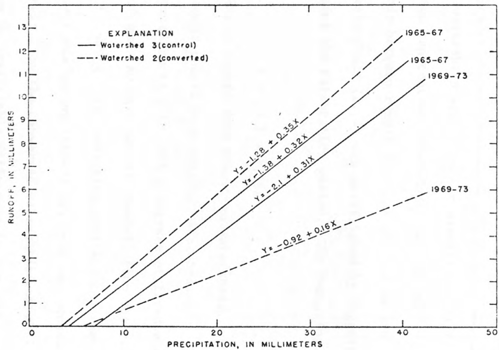
Figure 13.--Regression of precipitation ( X ) versus runoff ( Y ) from rainstorms at watersheds 2 and 3, Boco Mountain.
