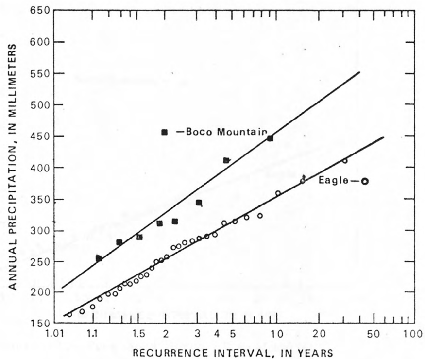
Figure 10.--Frequency curve of annual precipitation at Eagle and an estimated curve for Boco Mountain which is 30 percent larger.
