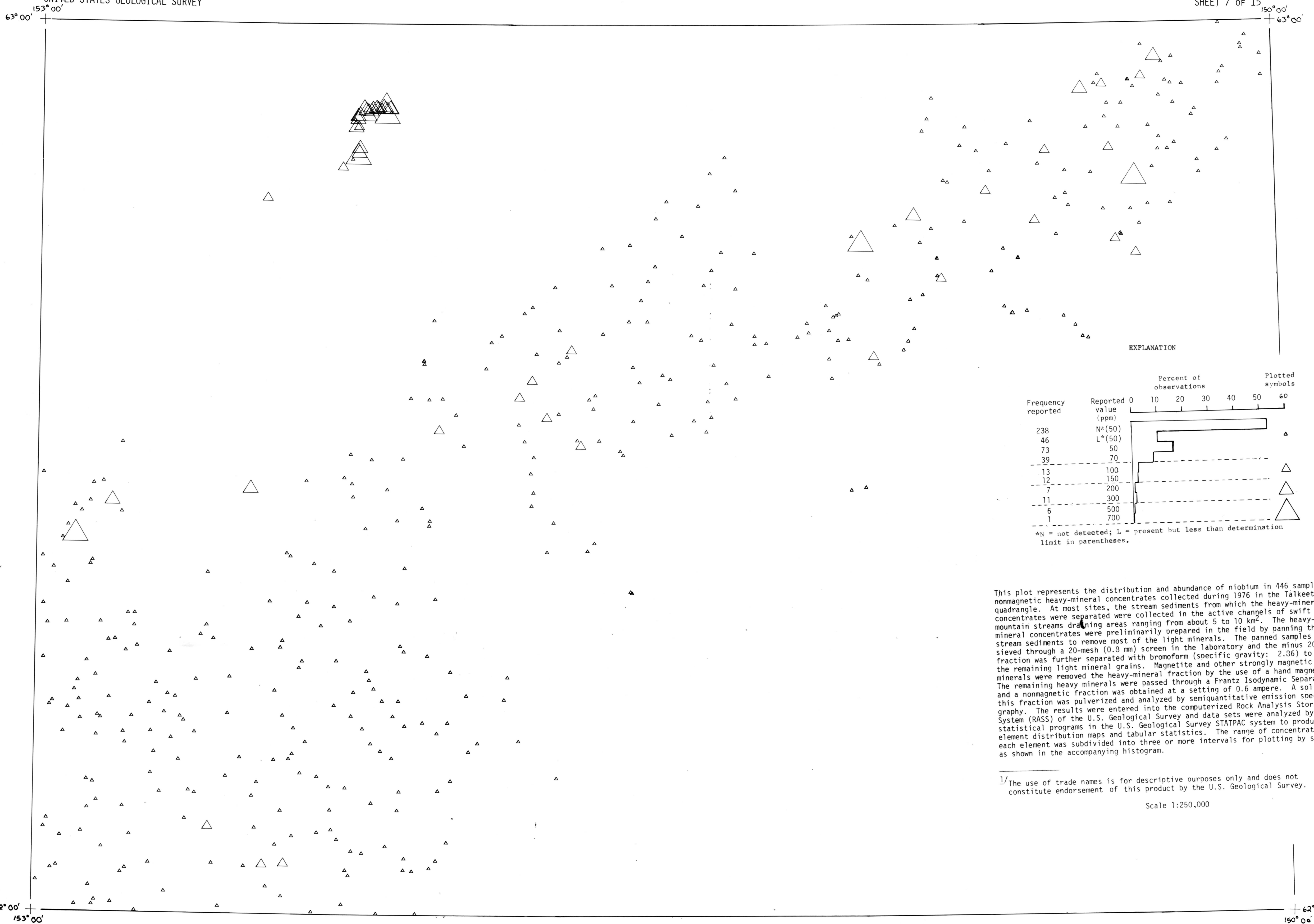
MAP SHOWING DISTRIBUTION PATTERN OF NIOBIUM IN NONMAGNETIC HEAVY MINERAL CONCENTRATE SAMPLES
