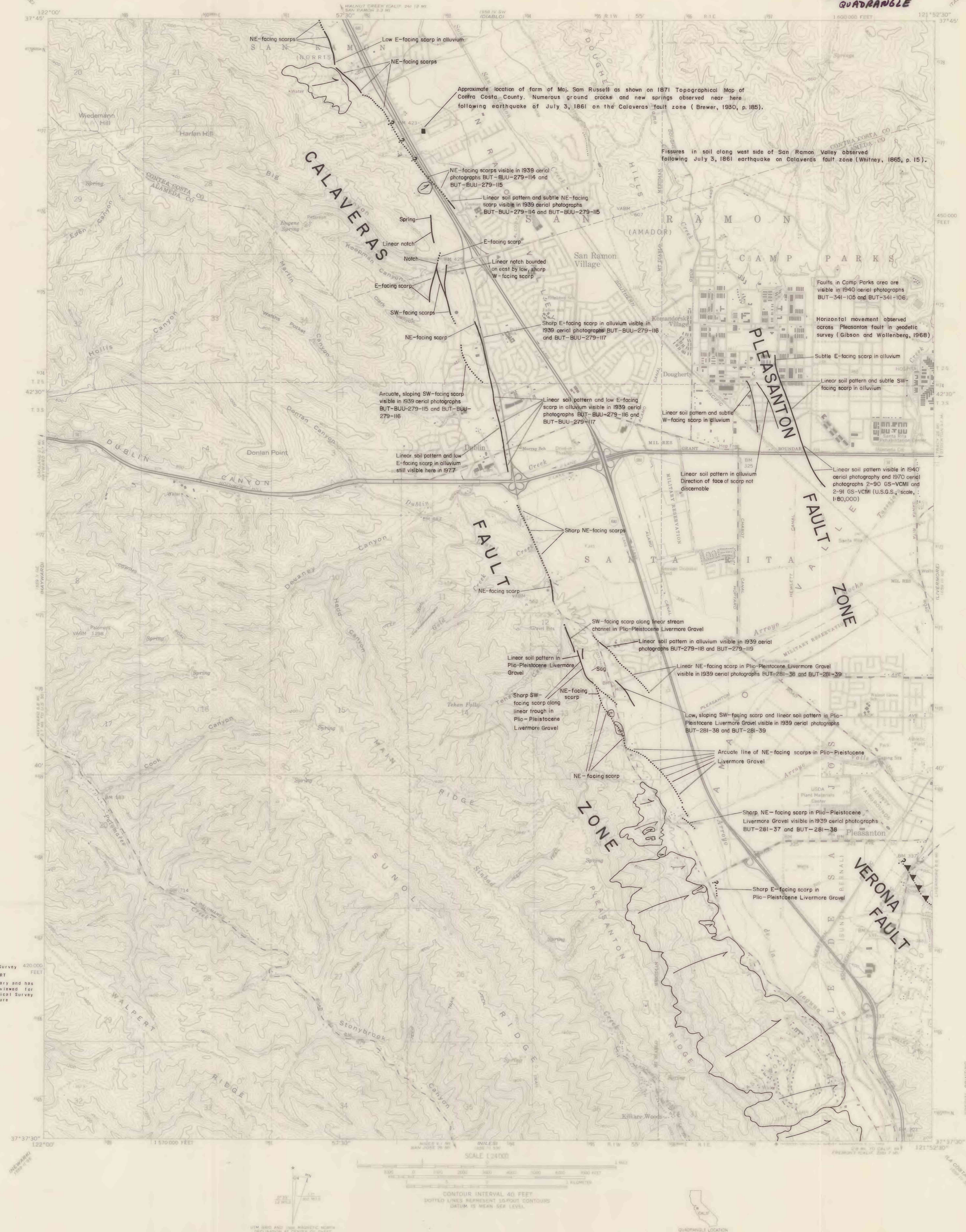
MAP OF QUATERNARY FAULTING ALONG THE NORTHERN CALAVERAS FAULT ZONE
