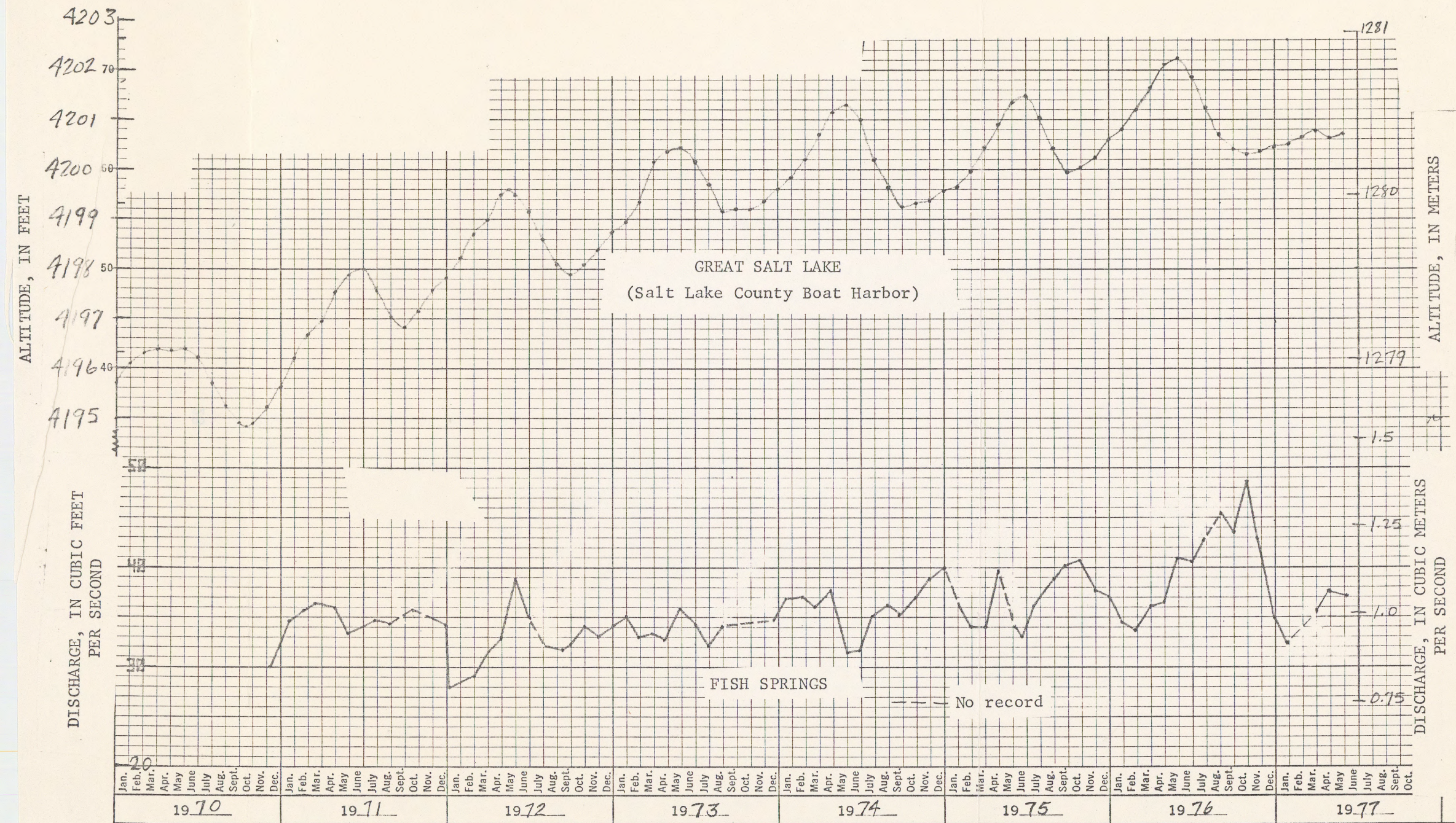
Figure 4.--Discharge of the eight largest springs in the Fish Springs group and fluctuation of Great Salt Lake, 1970-77.
