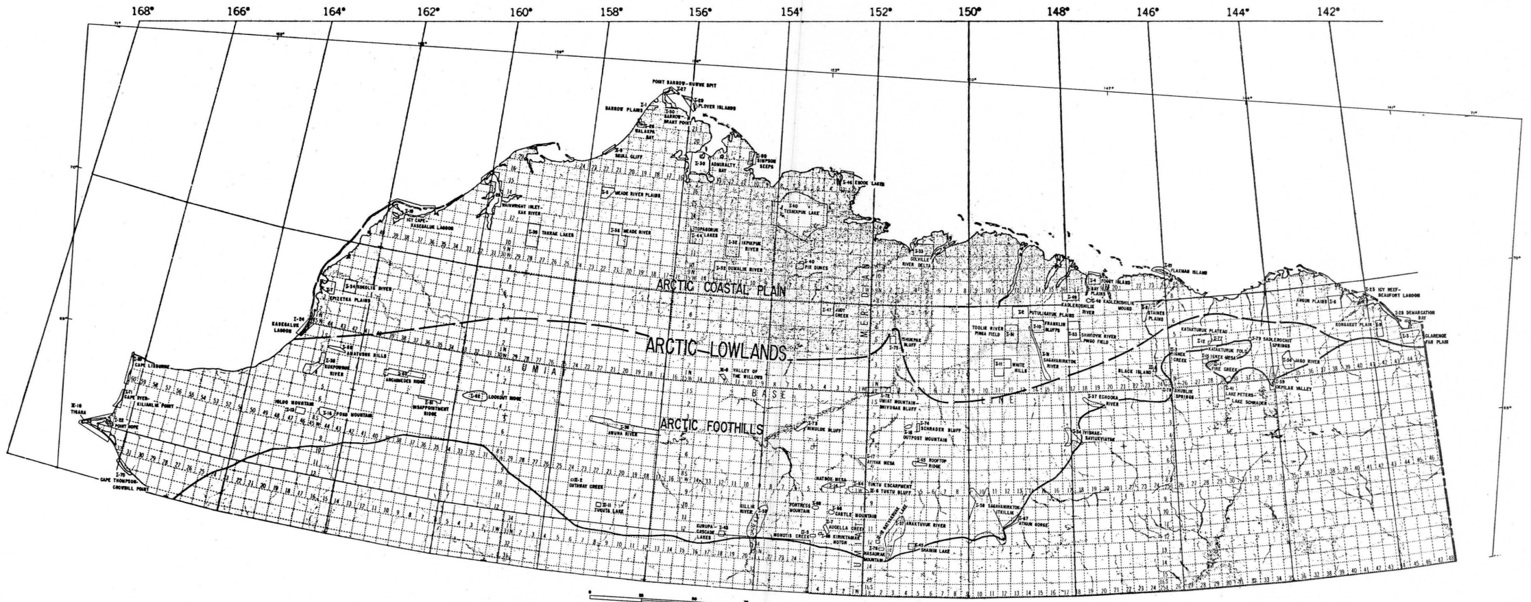
Figure 3 POTENTIAL NATURAL LANDFORM AND LIFEFORM LANDMARKS IN THE ARCTIC LOWLAND
