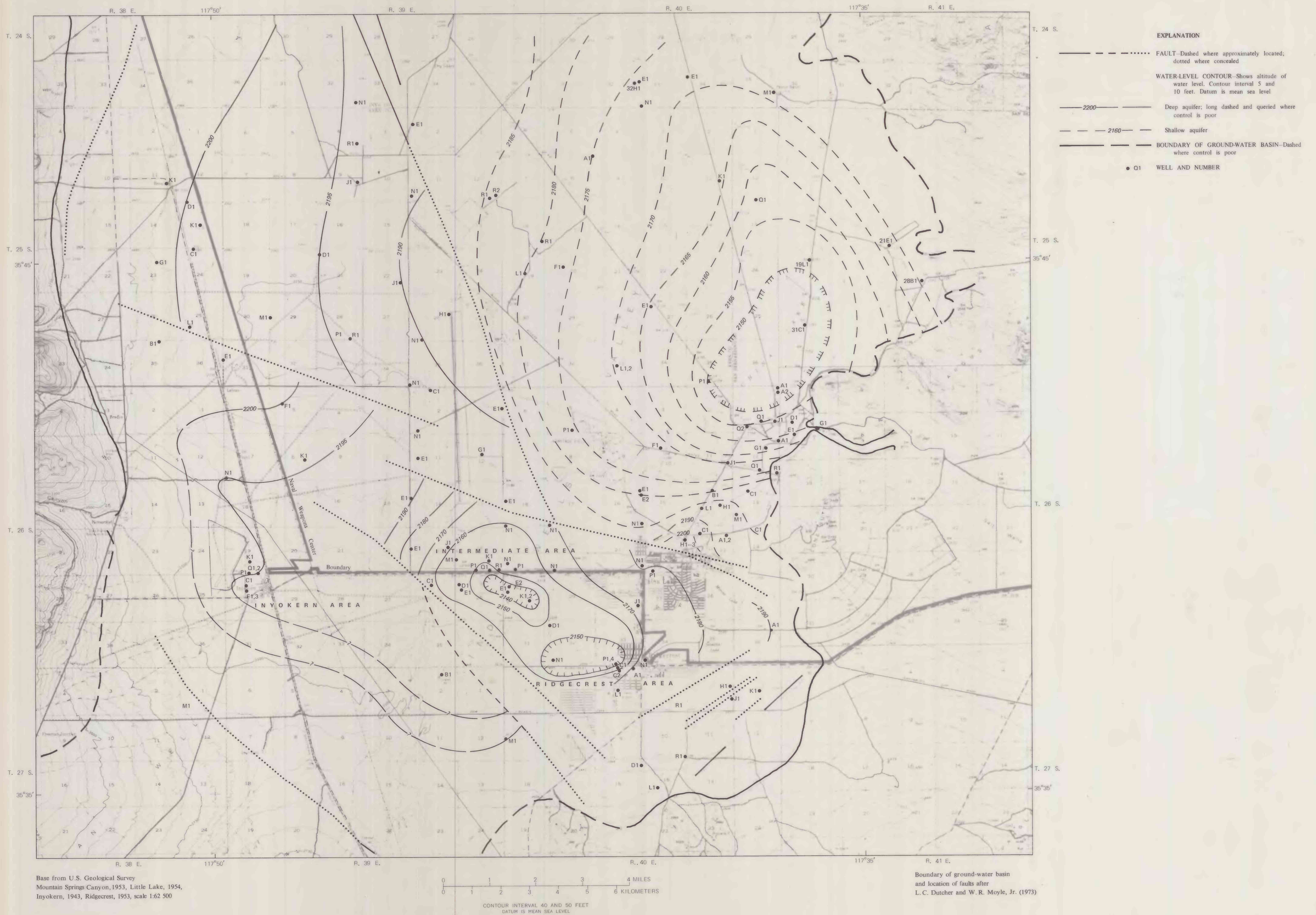
MAP OF INDIAN WELLS VALLEY, CALIFORNIA, SHOWING FAULTS, WATER-LEVEL CONTOURS, 1976, AND LOCATION OF OBSERVATION WELLS
