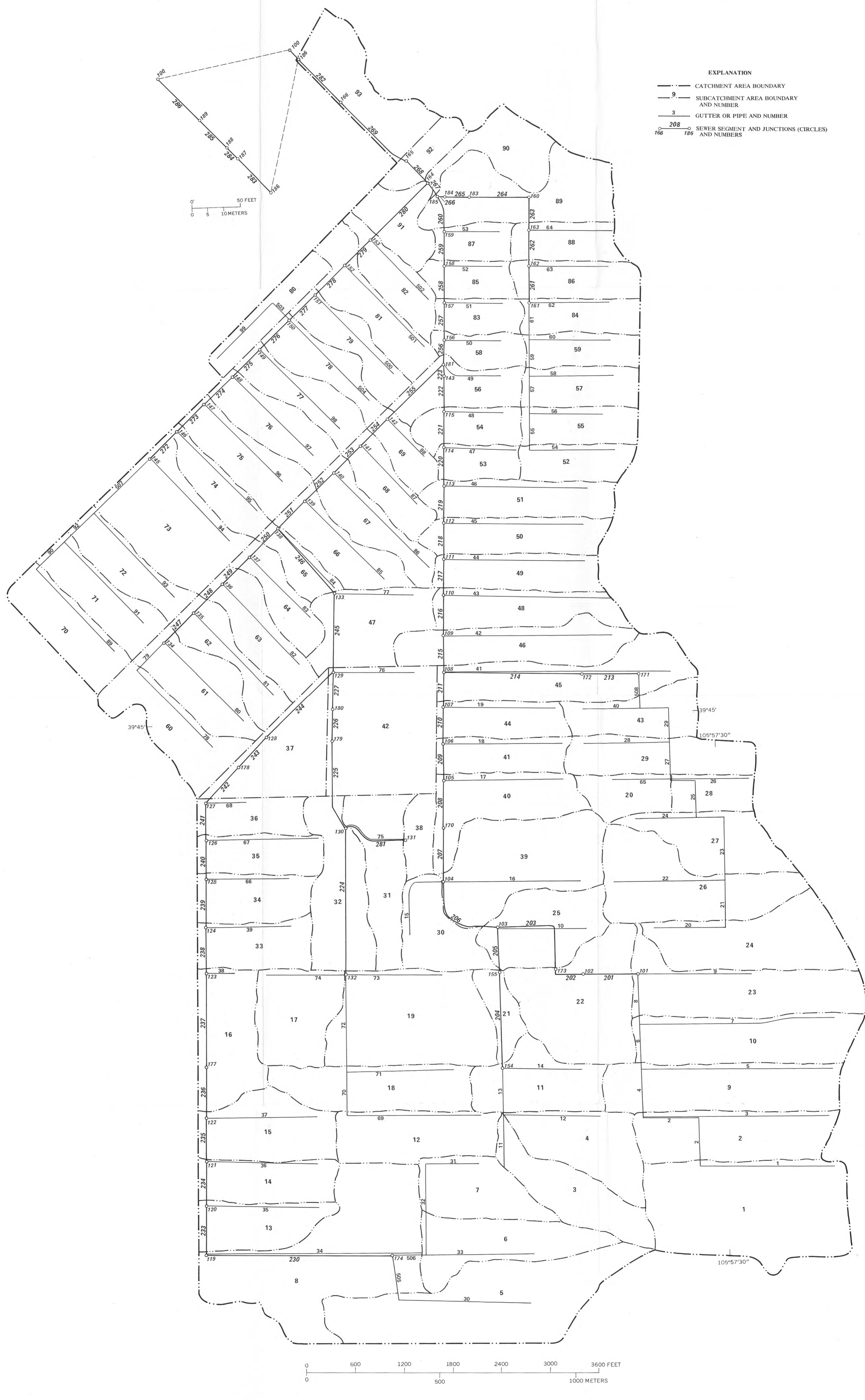
SCHEMATIC MAP SHOWING FEATURES RELATED TO USE OF STORM WATER MANAGEMENT MODEL II FOR THE CATCHMENT AREA DRAINED BY STORM SEWER AT THIRTY-SIXTH STREET, DENVER, COLORADO
