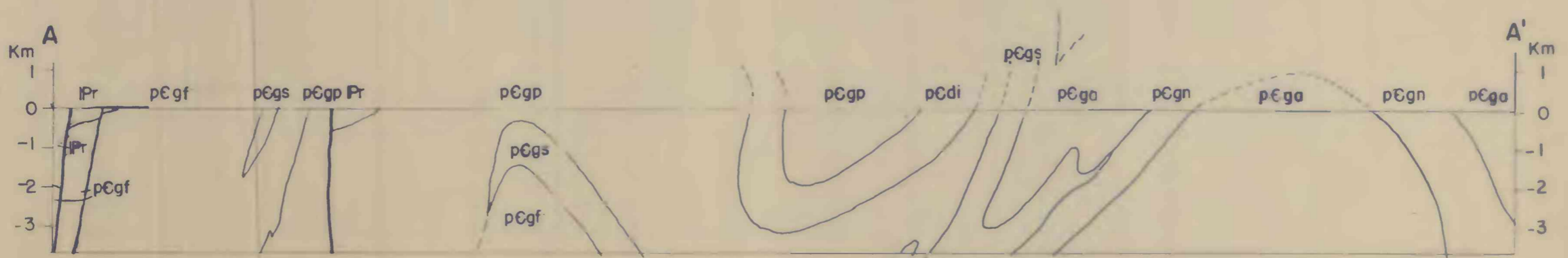
CROSS SECTION TO ACCOMPANY GEOLOGIC MAP
