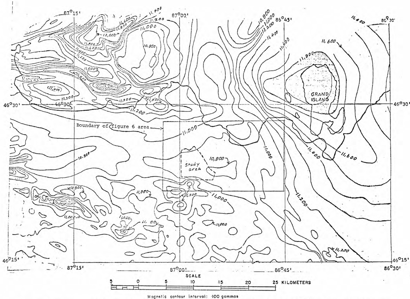
Figure 7.--Aeromagnetic map of part of Michigan, which includes the Rock River Canyon Wilderness Study Area (from Zietz and Kirby, 1971). Shows total intensity magnetic field of the earth in gammas relative to an arbitrary datum.
