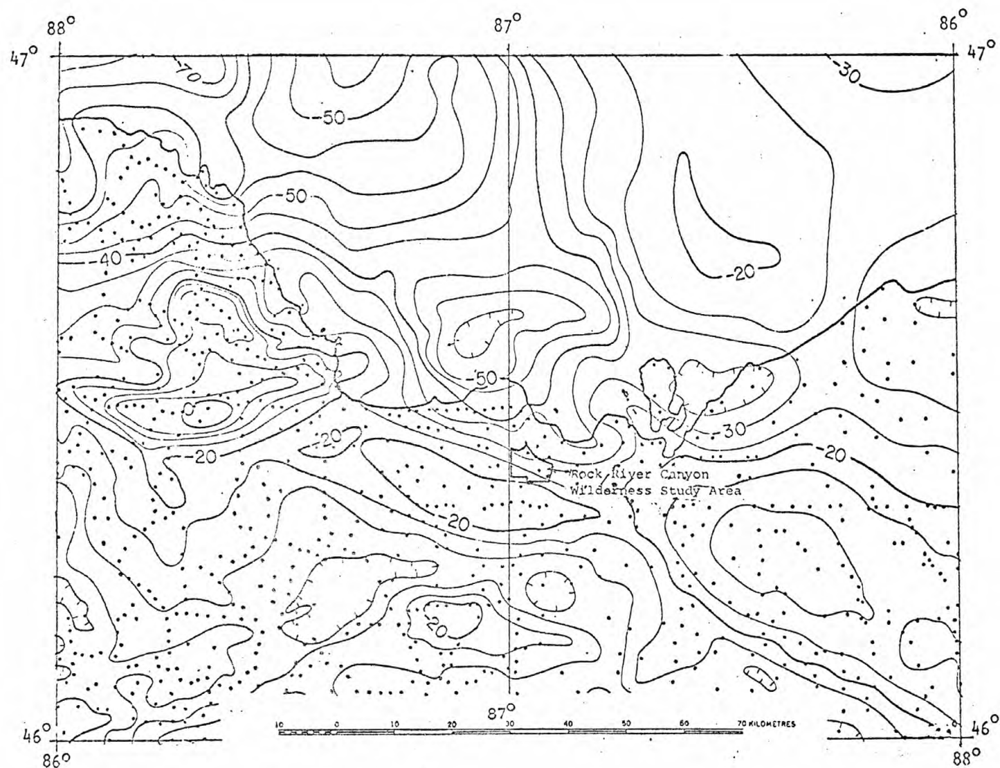
Figure 8. Portion of the Bouguer gravity map of the northern Michigan-Lake Superior area (Klasner and others, 1978). Contour interval 5 milligals. Station locations are shown by dots.
