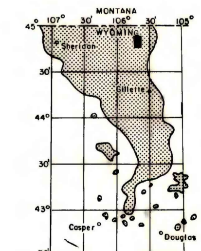
MAP SHOWING LOCATION OF THE HOMESTEAD DRAW SW QUAD- RANGLE AND THE POWDER RIVER BASIN KNOWN RECOVERABLE RESOURCE AREA (STIPPLED), WYOMING
