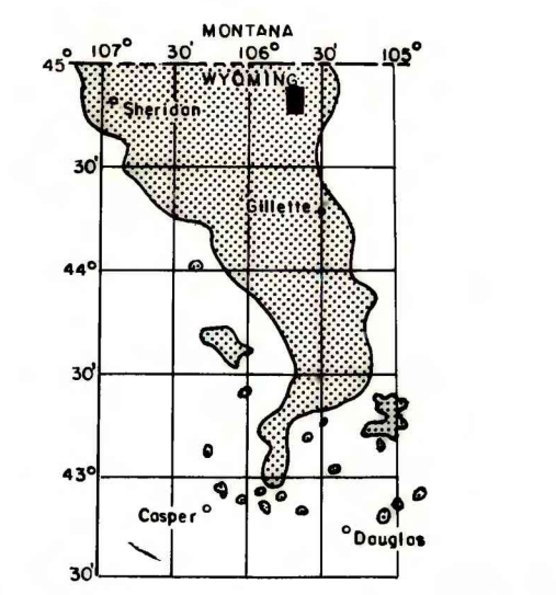
MAP SHOWING LOCATION OF THE HOMESTEAD DRAW SW QUADRANGLE AND THE POWDER RIVER BASIN KNOWN RECOVERABLE COAL RESOURCE AREA (STIPPLED), WYOMING
