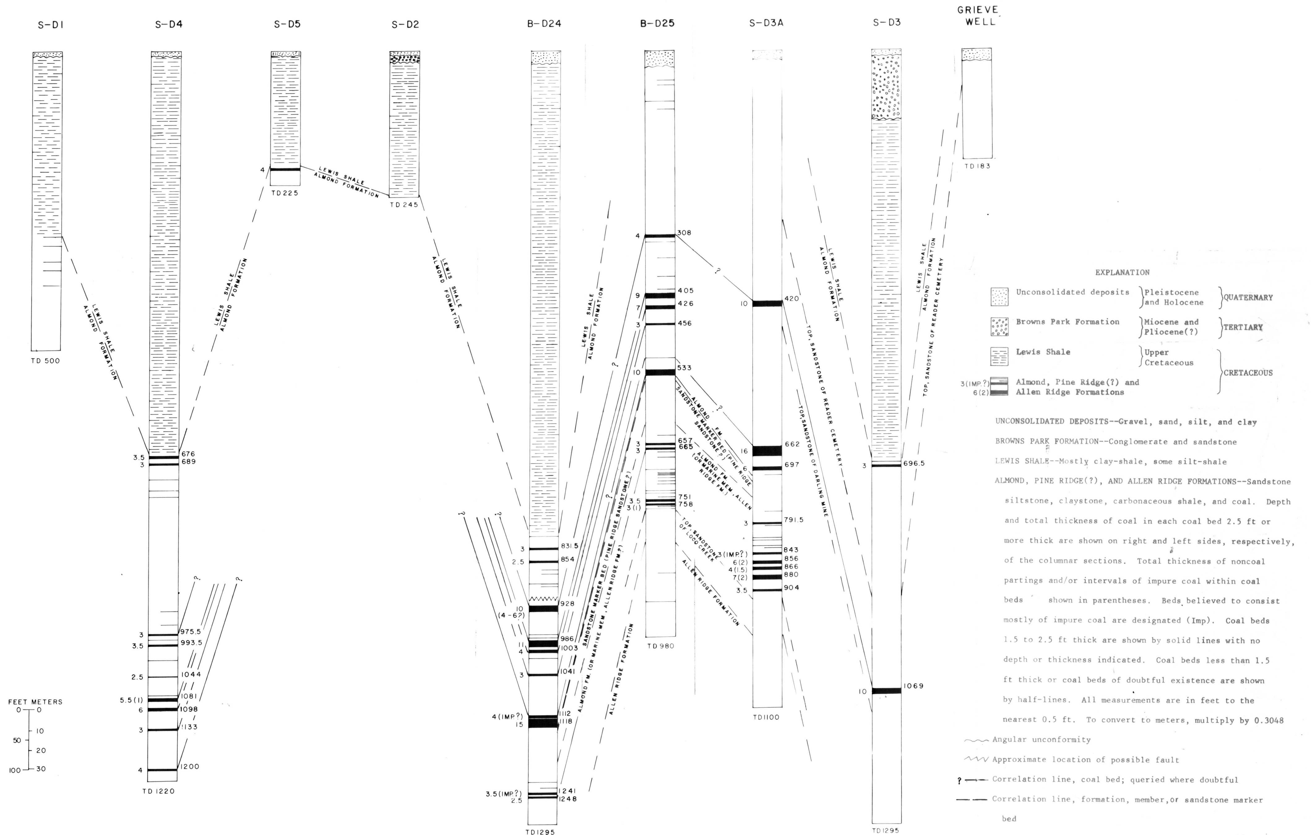
FIGURE 4. STRATIGRAPHIC SECTIONS OF HOLES DRILLED IN THE LEWIS SHALE, PINE RIDGE SANDSTONE (?), AND ALLEN RIDGE FORMATION.
