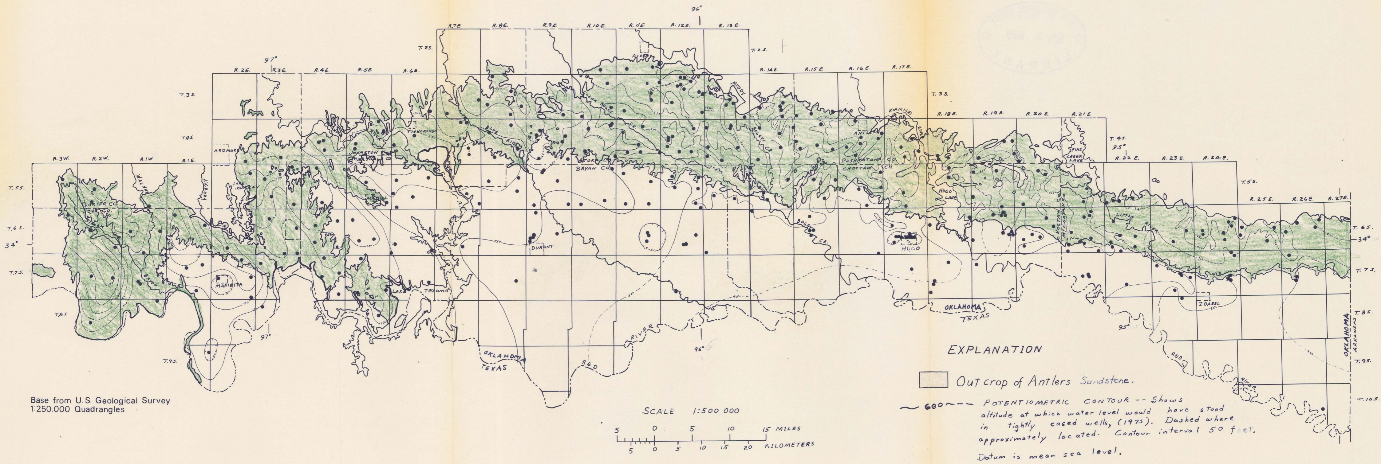
Figure 10. -- Potentiometric map of the Antlers aquifer, 1975.
