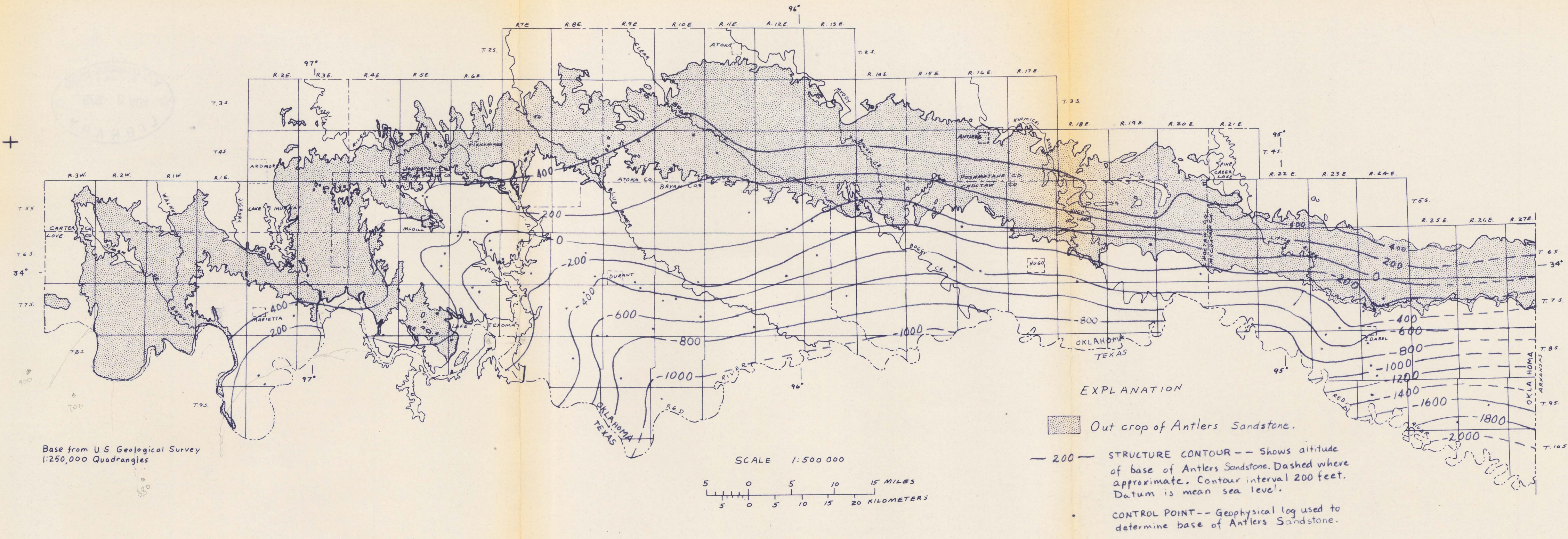
Figure 5.-- Structure-contour map showing the base of the Antlers Sandstone.
