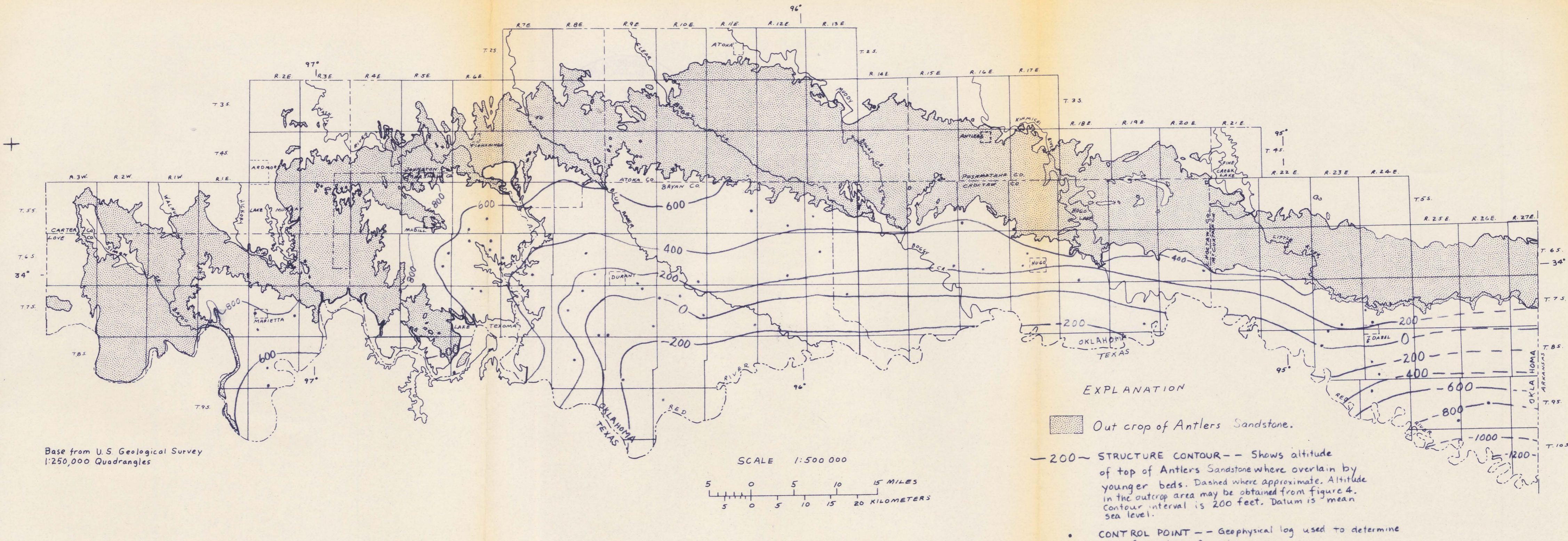
Figure 6. -- Structure-contour map showing the top of the Antlers Sandstone.
