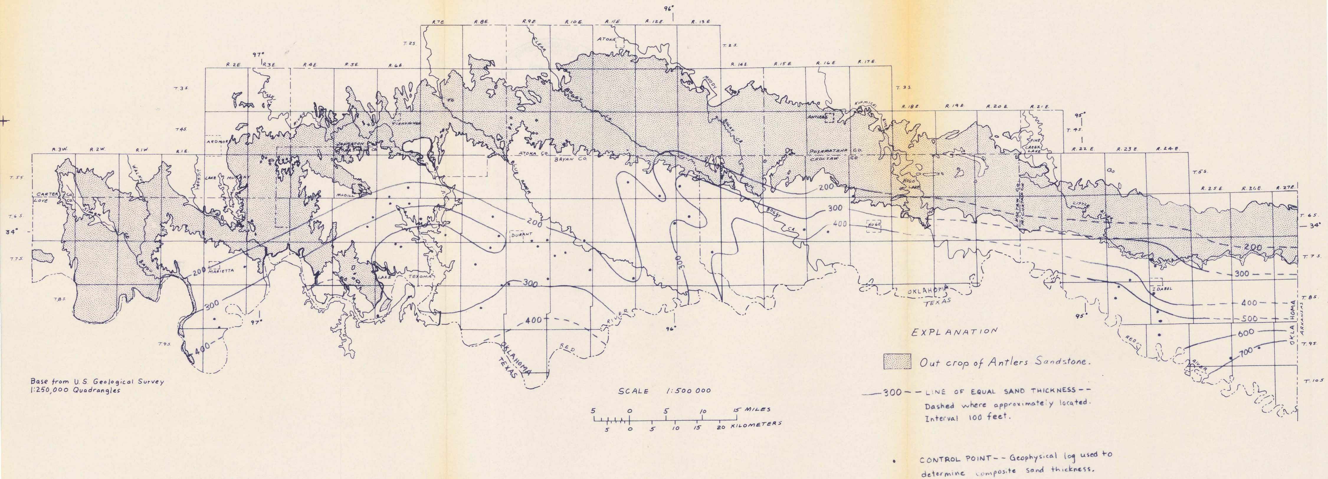
Figure 9.-- Map showing composite sand thickness of the Antlers Sandstone.
