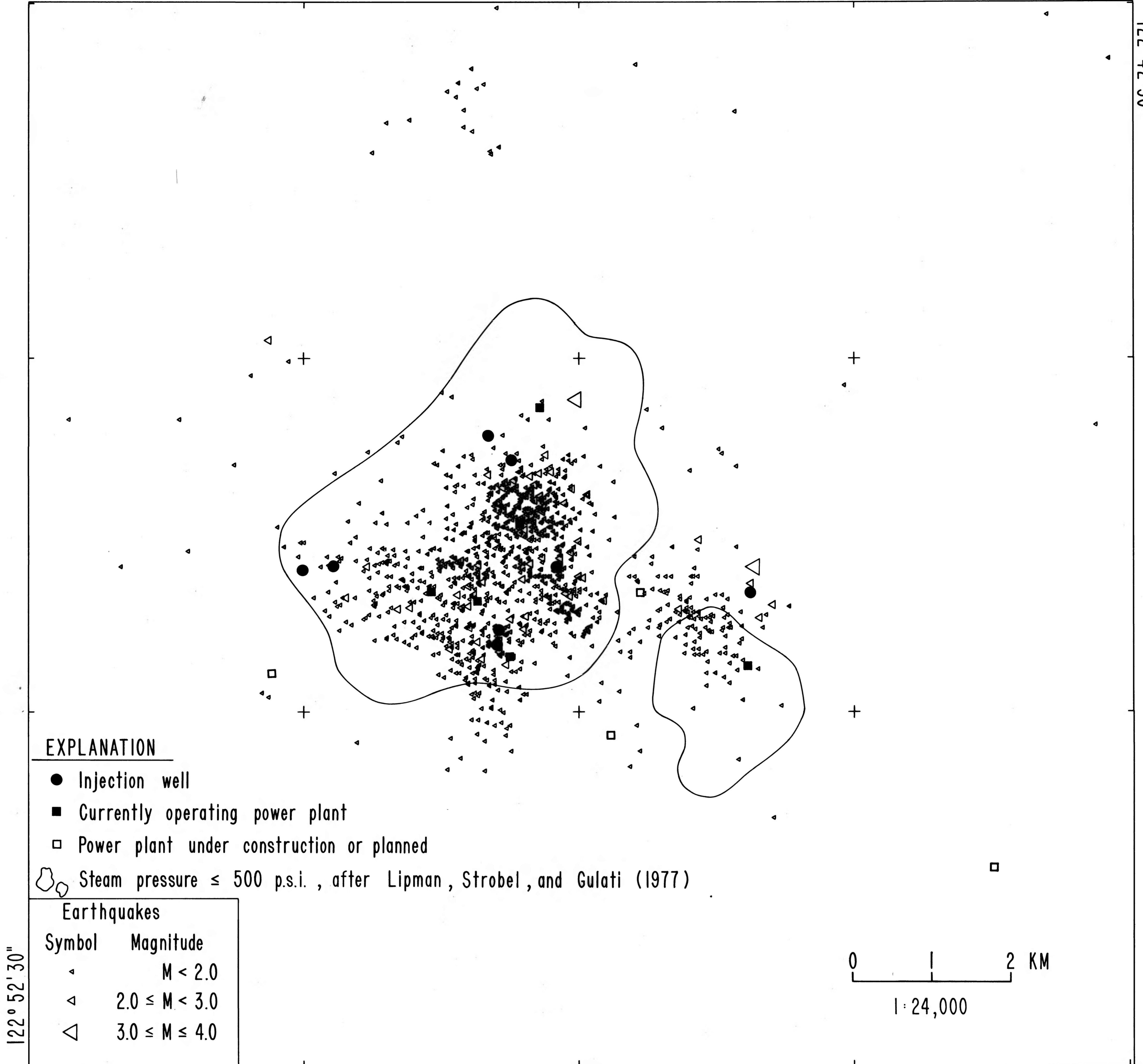
INJECTION WELLS, POWER PLANTS AND PRELIMINARY HYPOCENTERS OF EARTHQUAKES (JUN. 1975 - SEPT. 1977)
