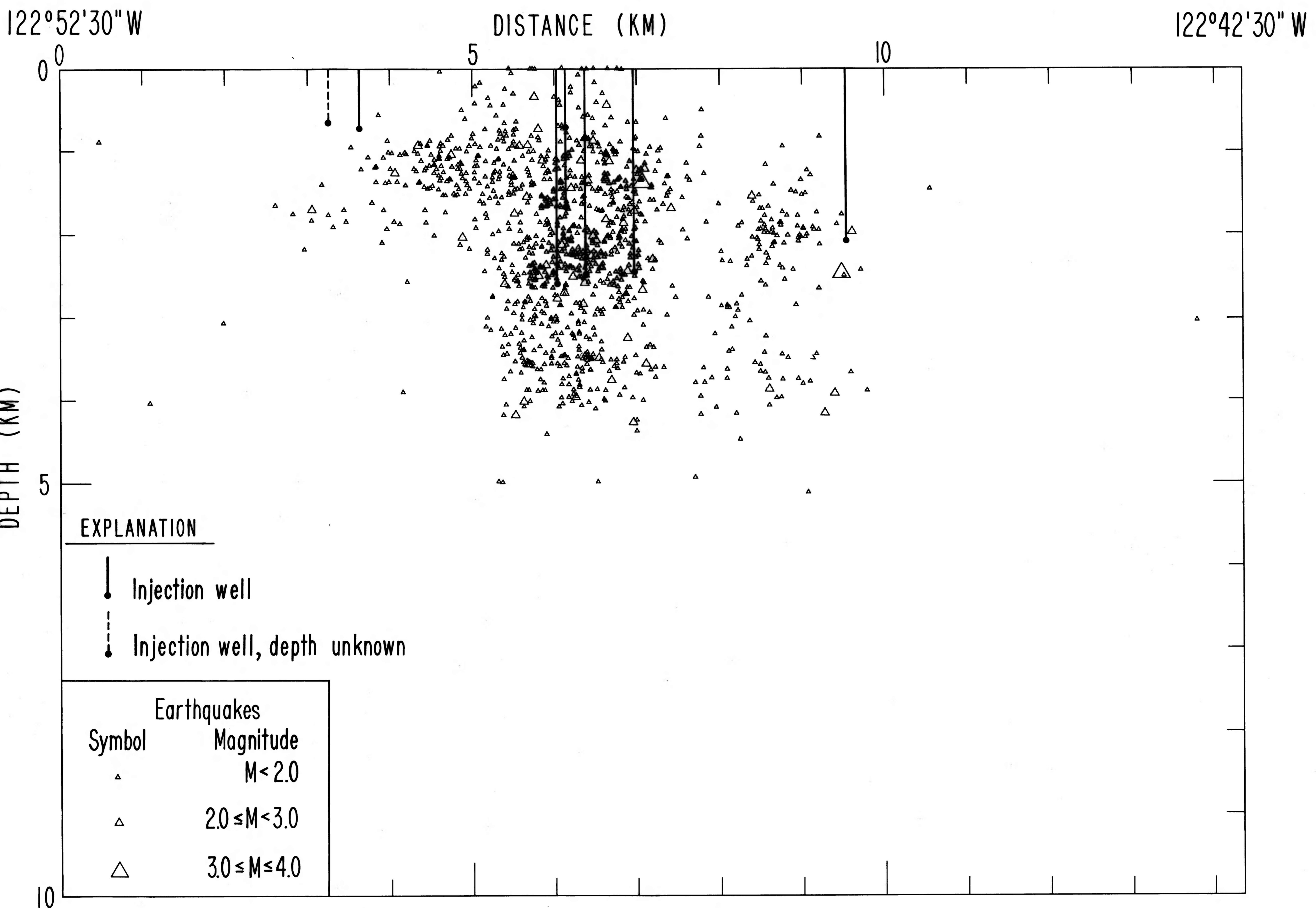
N 90° E CROSS SECTION THROUGH PRODUCTION ZONE (Latitude 38° 46' N to 38° 51' N)
