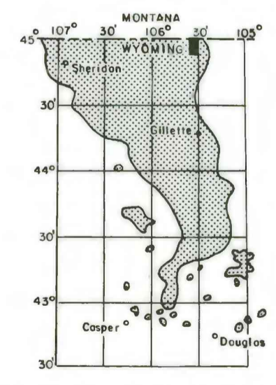
MAP SHOWING LOCATION OF THE HOMESTEAD DRAW QUADRANGLE AND THE POWDER RIVER BASIN KNOWN RECOVERABLE COAL RESOURCE AREA (STIPPLED), WYOMING
