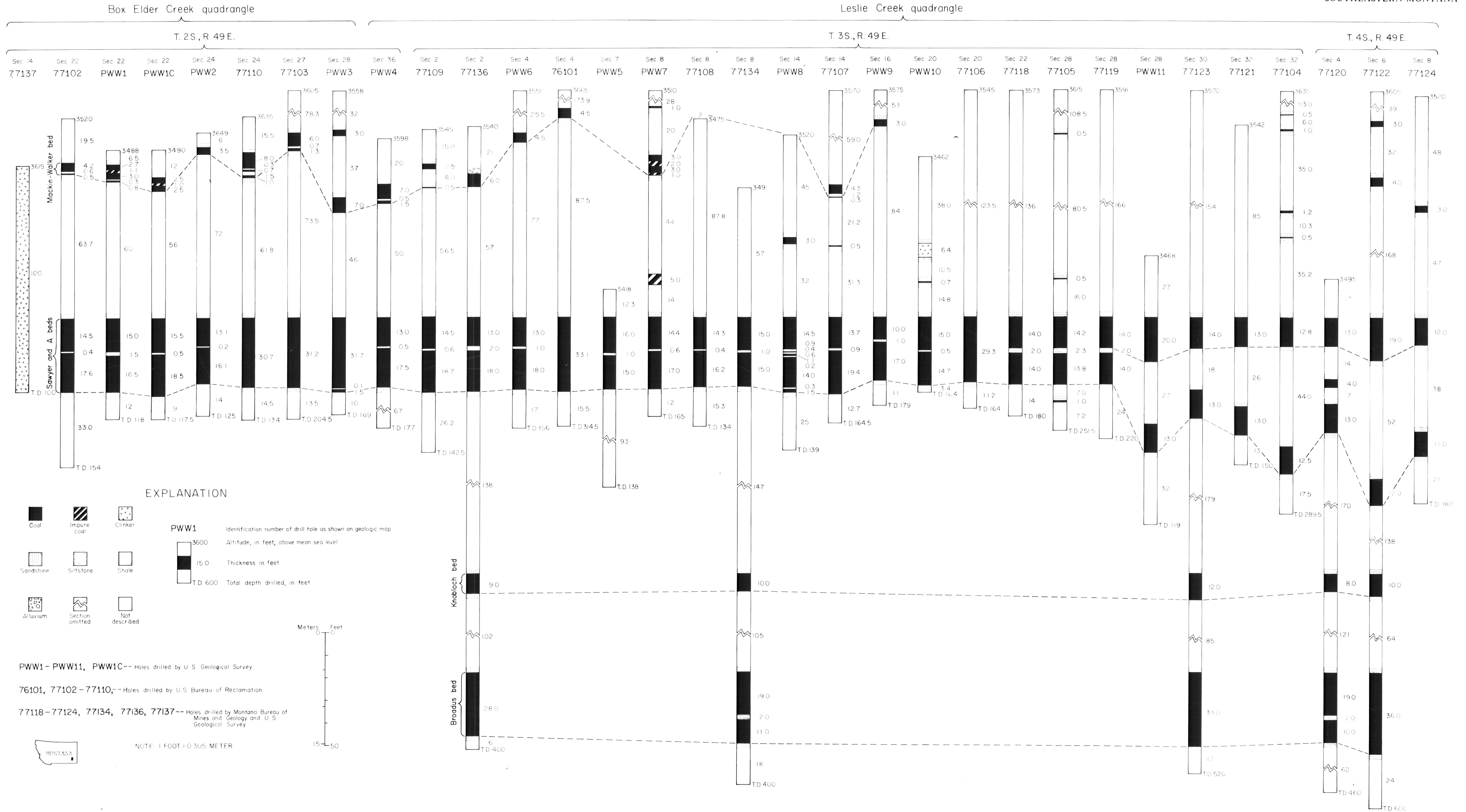
Coal beds in exploration holes drilled in Pumpkin Creek EMRIA Study Site, Box Elder Creek and Leslie Creek quadrangles, Powder River County, Montana
