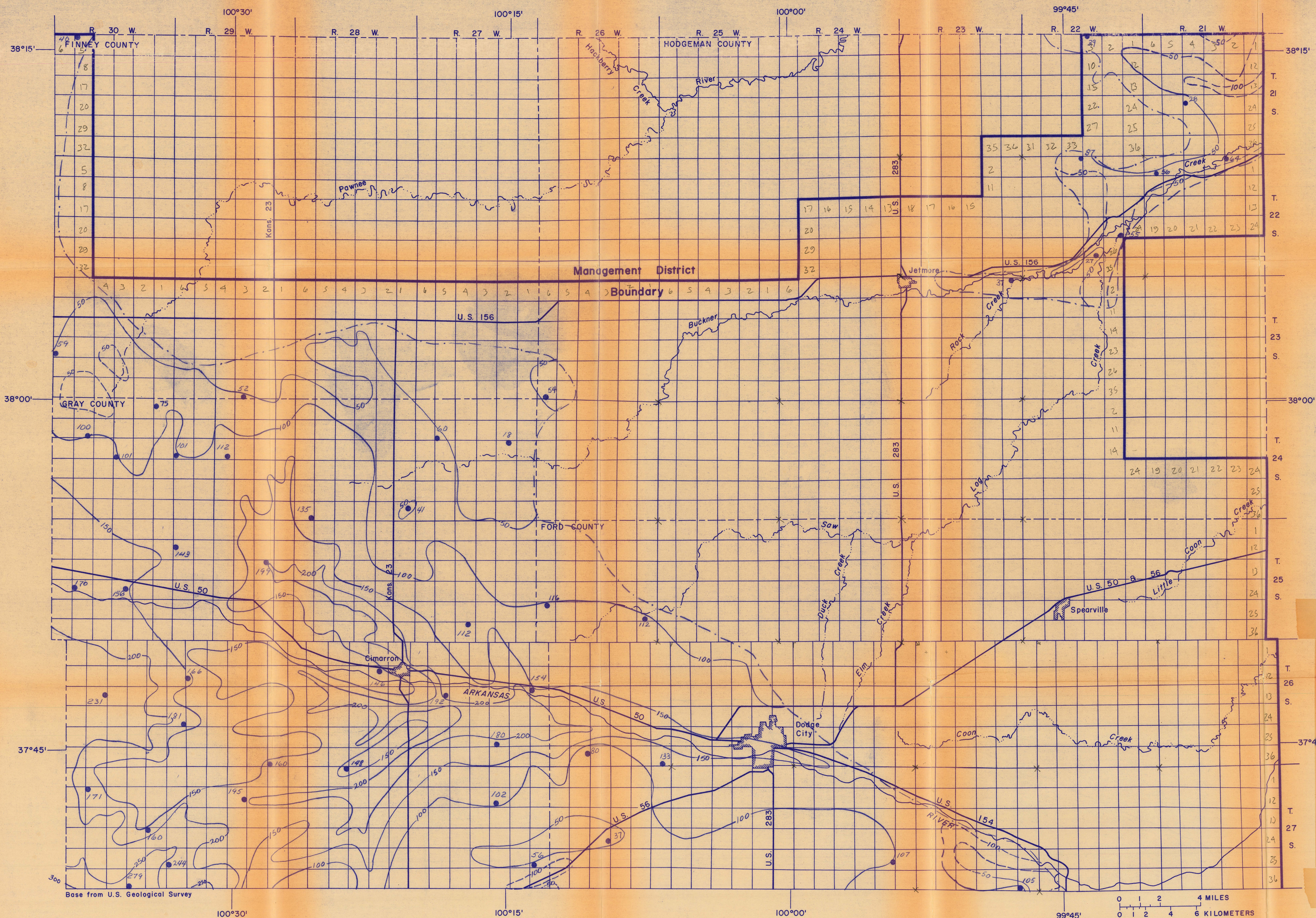
MAP SHOWING SATURATED THICKNESS OF THE UNCONSOLIDATED AQUIFER, SOUTHWESTERN KANSAS, JANUARY 1978
