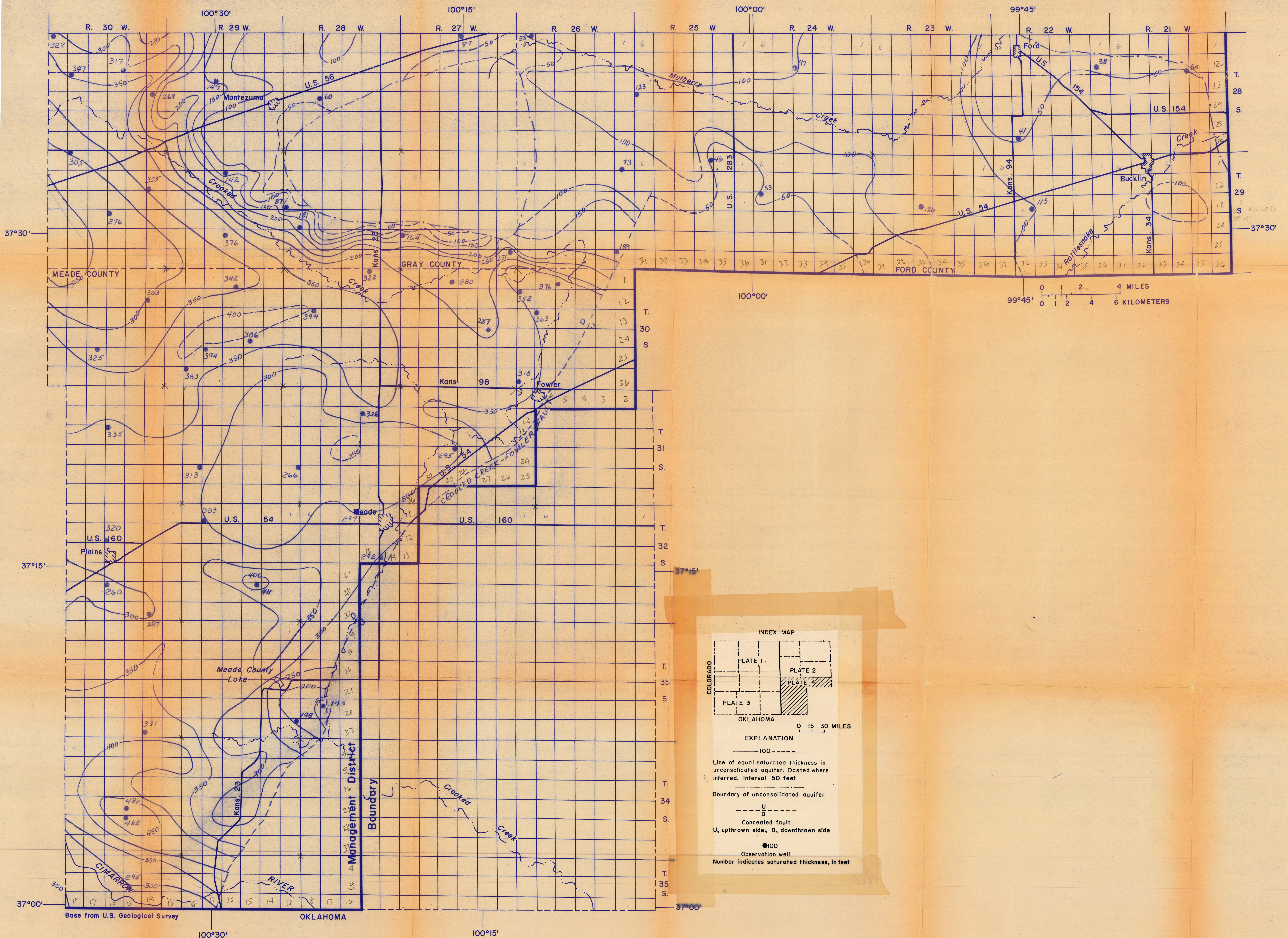
MAP SHOWING SATURATED THICKNESS OF THE UNCONSOLIDATED AQUIFER, SOUTHWESTERN KANSAS, JANUARY 1978
