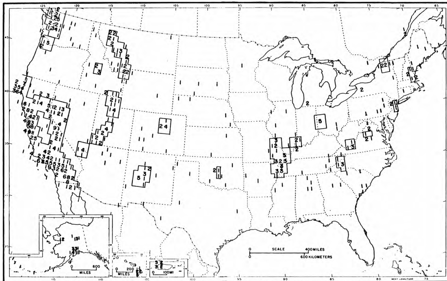
Fig. 2 - NUMBERS OF EVENTS OF MODIFIED MERCALLI INTENSITY VI OR GREATER, 1870 - 1970, AND REGIONS OF PROBABLE STRONG GROUND MOTION.
