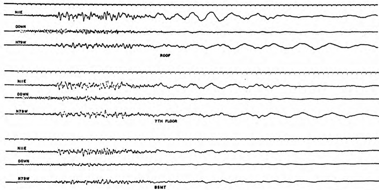
Fig. 8 - ACCELEROGRAPH RECORDS FROM 15250 VENTURA BLVD., SAN FERNANDO EARTHQUAKE FEBRUARY 9, 1971.
