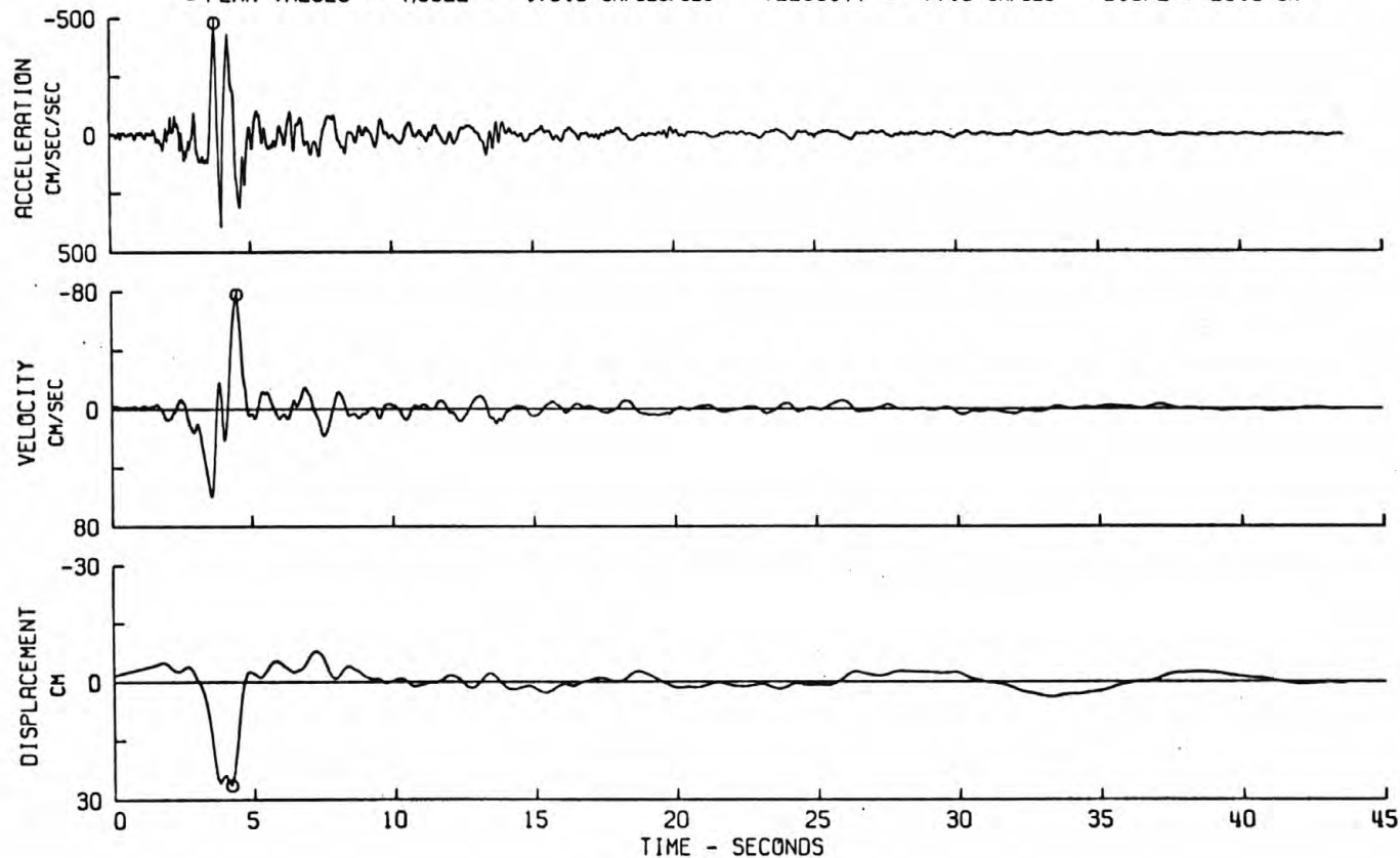
Fig. 4 - ACCELERATION, VELOCITY, & DISPLACEMENT TRACES FOR THE N65E COMPONENT OF MOTION AT CHOLAME-SHANDON STATION 2, PARKFIELD EARTHQUAKE, JUNE 27, 1966.
