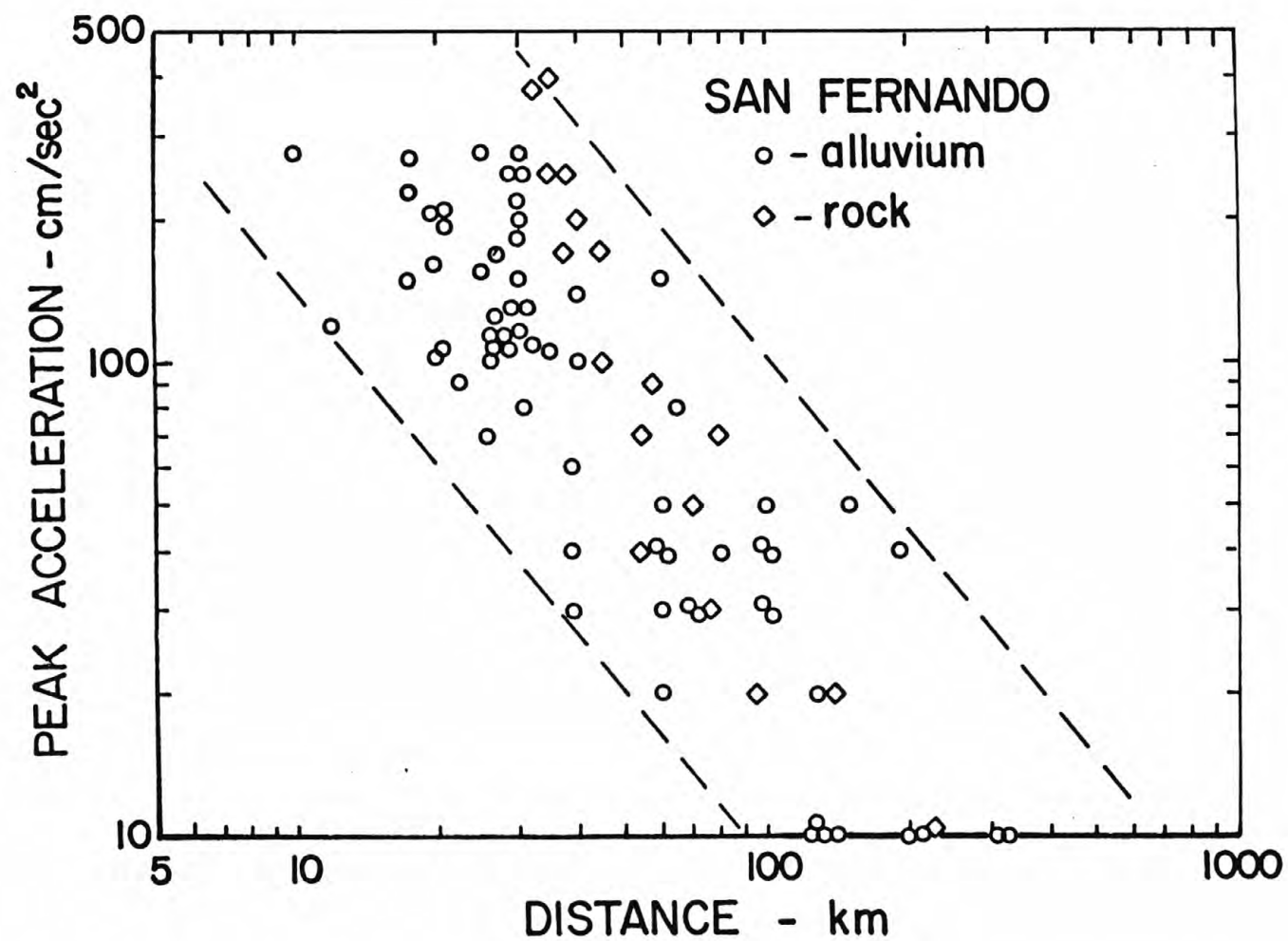
Fig. 5 - ATTENUATION OF PEAK ACCELERATION WITH DISTANCE, SAN FERNANDO EARTHQUAKE FEBRUARY 9, 1971.
