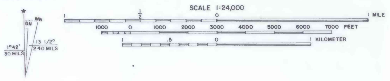
COAL RESOURCE OCCURRENCE MAP OF THE DUNN CENTER NW QUADRANGLE, DUNN COUNTY, NORTH DAKOTA BY WOODWARD-CLYDE CONSULTANTS 1978
