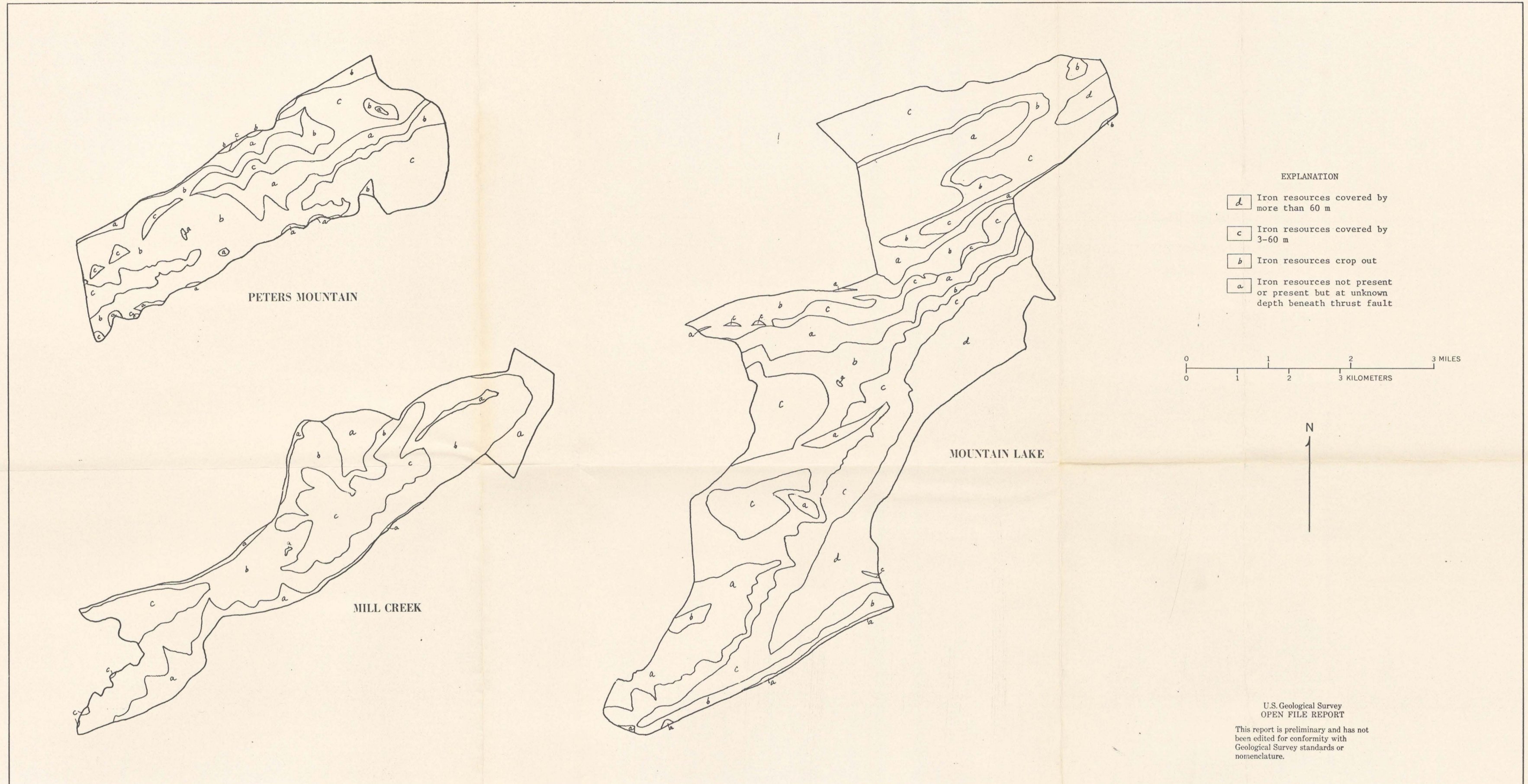
MAPS SHOWING AREAS OF EXPOSED AND CONCEALED IRON RESOURCES IN HEMATITIC SANDSTONE OF THE ROSE HILL FORMATION, MILL CREEK, MOUNTAIN LAKE, AND PETERS MOUNTAIN WILDERNESS STUDY AREAS
