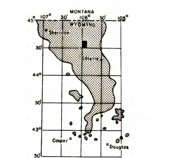
MAP SHOWING LOCATION OF THE CROTON QUADRANGLE AND THE POWDER RIVER BASIN KNOWN RECOVERABLE COAL RESOURCE AREA (STIPPLED), WYOMING
